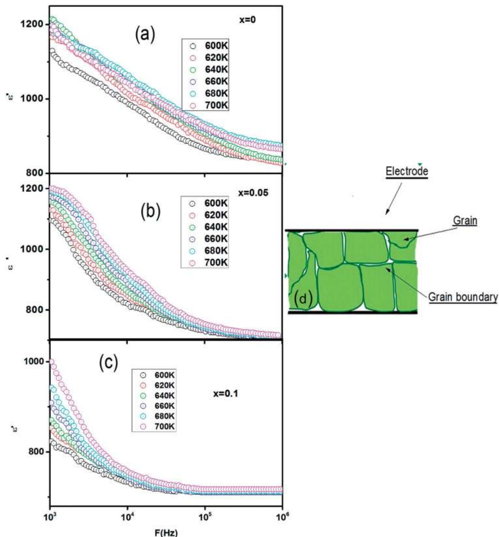
Fig. 2 (a–c): frequency dependence of real ( \epsilon' ) part of permittivity of \text{CETCo}_x for x = 0.00, 0.05 and 0.10 . (d): is a schematic structure of the samples.
