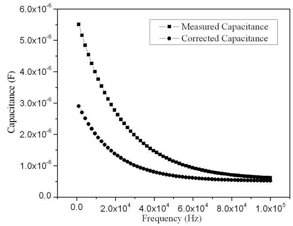
Fig. 5. The frequency dependent plot of corrected capacitance.
