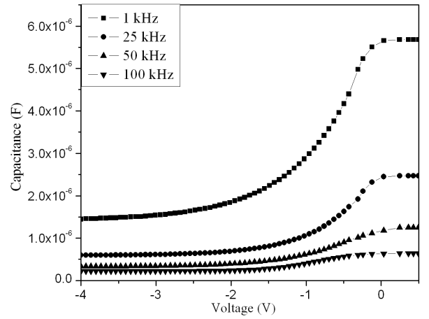
Fig. 1. C - V curves of the Au/ n -Si/CuPc/Au heterostructure at different frequency.
