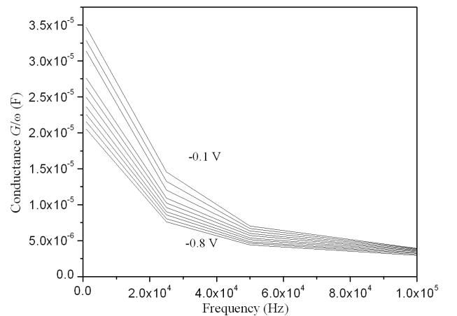
Fig. 3. G/\omega - f characteristics of Au/ n -Si/CuPc/Au structure at different biases.
