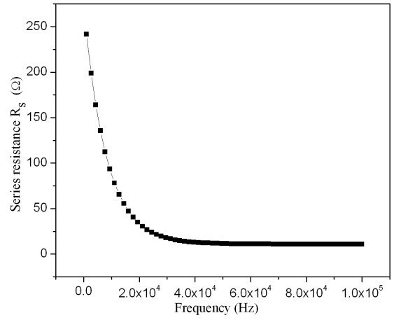
Fig. 4. Series resistance vs. frequency plot of Au/n-Si/CuPc/Au heterostructure.
