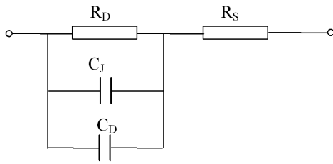
Fig. 7. Equivalent circuit diagram of Au/ n -Si/CuPc/Au heterostructure.
