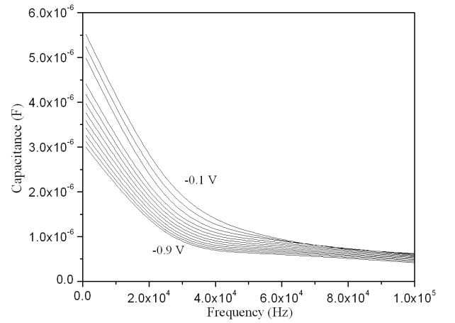
Fig. 2. C - f characteristics of Au/ n -Si/CuPc/Au structure at different biases.
