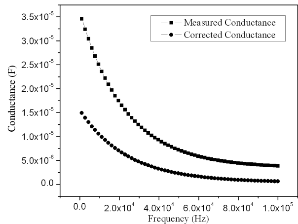
Fig. 6. The frequency dependent plot of corrected conductance.
