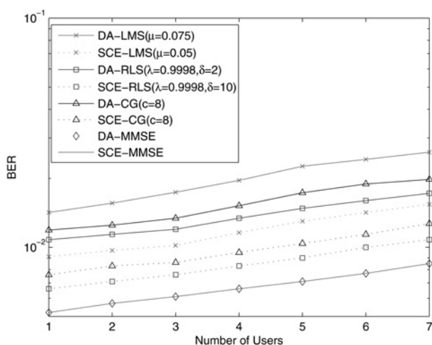
Figure 8 BER performance of the proposed SC-FDE detection schemes against the number of users in the scenario with a 16 dB SNR
