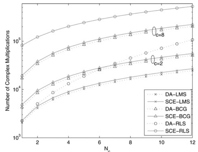
Figure 2 Complexity comparison of the proposed schemes
