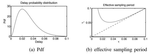
Fig. 3. Delay probability density and average (effective) control update period as a function of sampling period \tau
