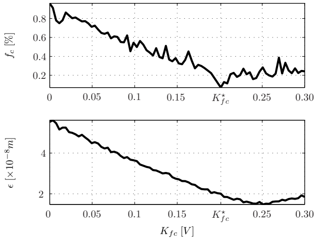
Fig. 6. PERFORMANCE Performance in time and frequency domain. Linearity is measured by the cost function f_c(K_{fc}) in the frequency domain and time domain performance as defined in (7) (low gain feedback K_p = 5 \cdot 10^6 ).
