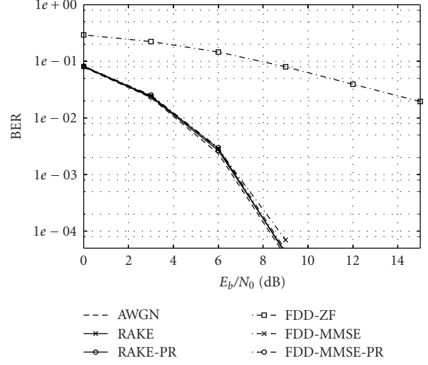
FIGURE 9: Performance comparison for PAM and PR-PAM, N_u = 1 ( N_c = 32, N_f = 64 ).
