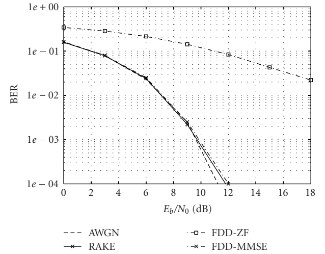
FIGURE 7: Performance comparison for PPM, N_u = 1 ( N_c = 16 , N_f = 64 ).
