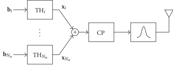
FIGURE 2: Block representation of the BT UWB-IR transmitter with cyclic prefix.
