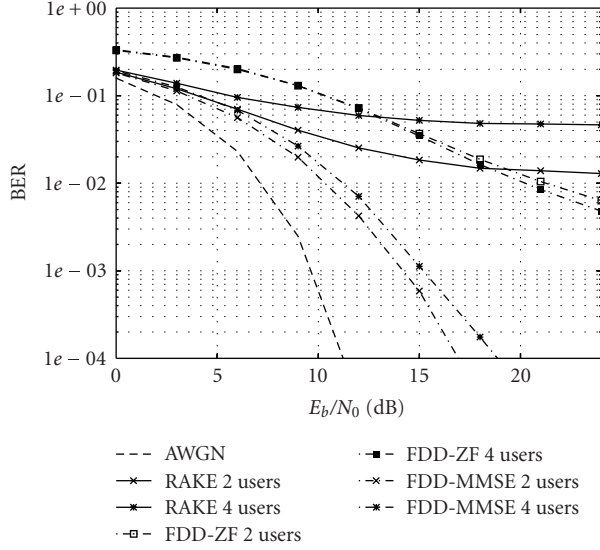
FIGURE 4: Performance comparison for PPM, N_u = 2 and N_u = 4 ( N_c = 4 , N_f = 4 ).
