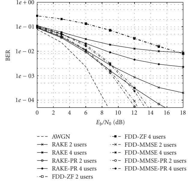
FIGURE 6: Performance comparison for PAM and PR-PAM, N_u = 2 and N_u = 4 ( N_c = 8 , N_f = 4 ).
