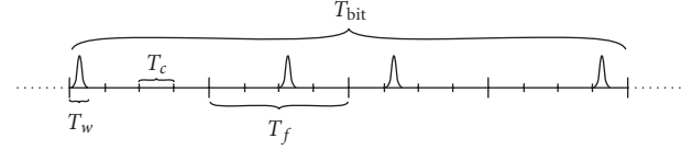
FIGURE 1: Representation of a transmitted bit. In the above example, b = 1 and c_\ell(m) = \{0, 2, 1, 3\} .
