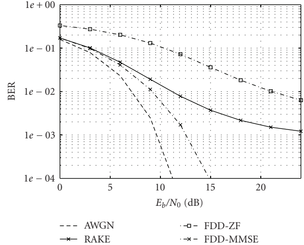
FIGURE 3: Performance comparison for PPM, N_u = 1 ( N_c = 4 , N_f = 4 ).
