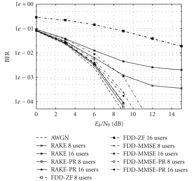
FIGURE 10: Performance comparison for PAM and PR-PAM, N_u = 8 and N_u = 16 ( N_c = 32, N_f = 64 ).
