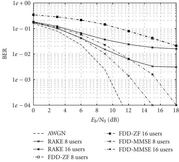
FIGURE 8: Performance comparison for PPM, N_u = 8 and N_u = 16 ( N_c = 16, N_f = 64 ).
