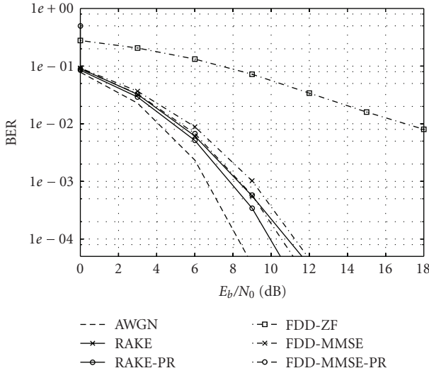
FIGURE 5: Performance comparison for PAM and PR-PAM, N_u = 1 ( N_c = 8 , N_f = 4 ).
