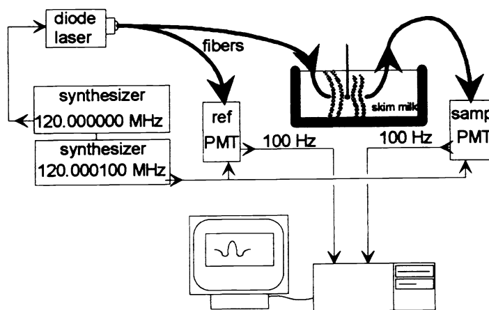
Fig. 1. Schematic of instrument.
