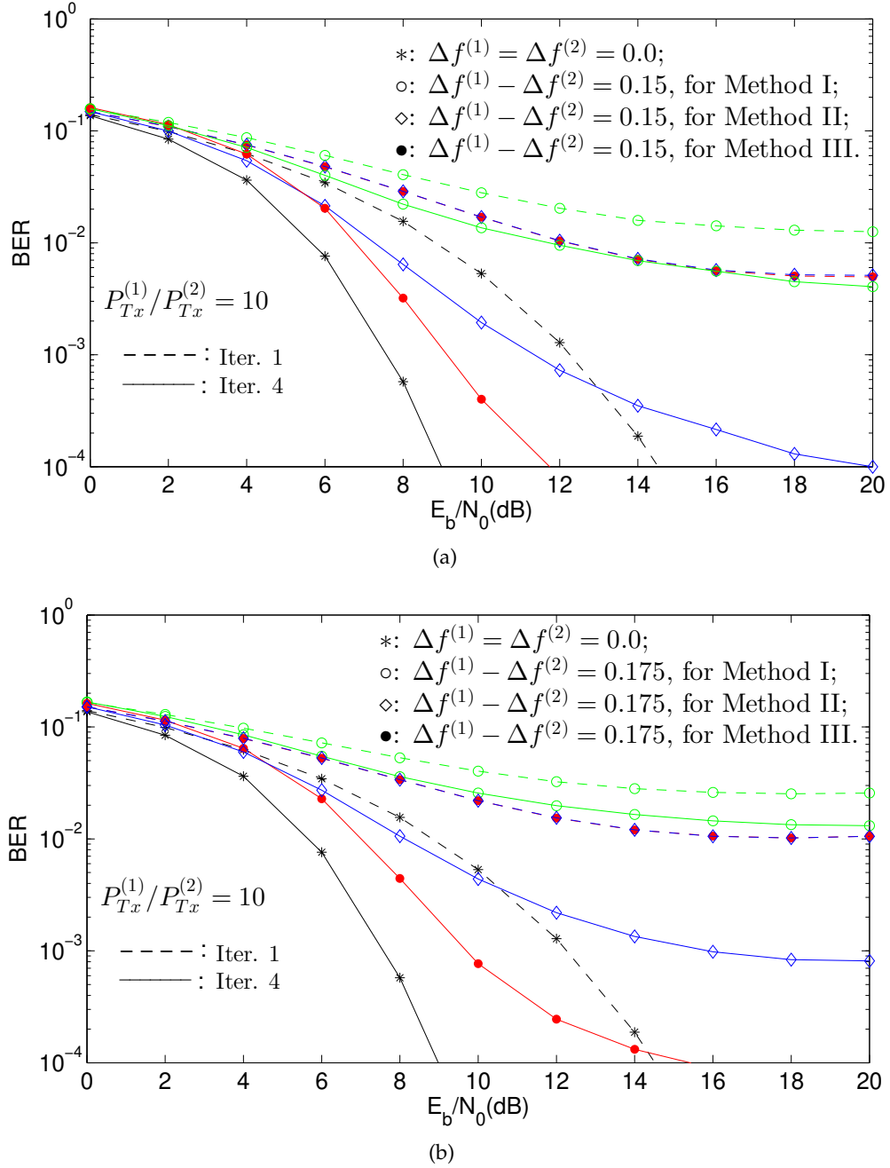
Figure 6.7: BER performance for the proposed methods, with a power relation of 10dBs between both transmitters, and considering values of: \Delta f^{(1)} - \Delta f^{(2)} = 0.15 (a); \Delta f^{(1)} - \Delta f^{(2)} = 0.175 (b).
