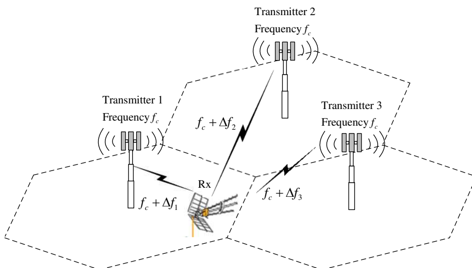
Figure 5.1: Single frequency network transmission.
