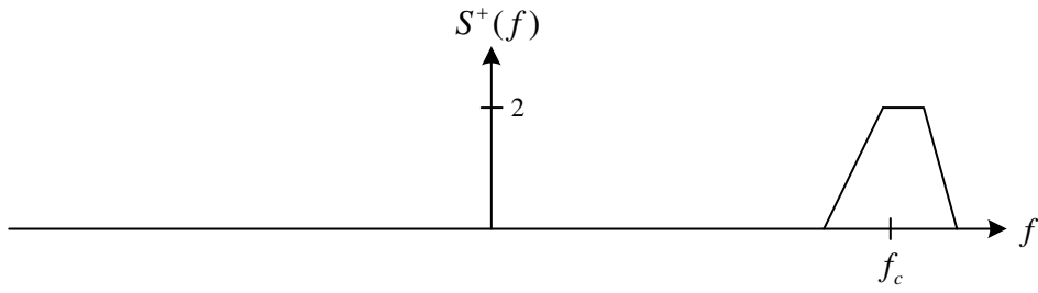
Figure B.2: The spectrum S^+(f)
