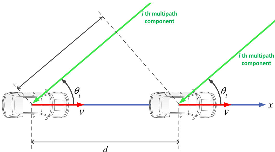
Figure 2.12: Difference in path lengths from the transmitter to the mobile station
