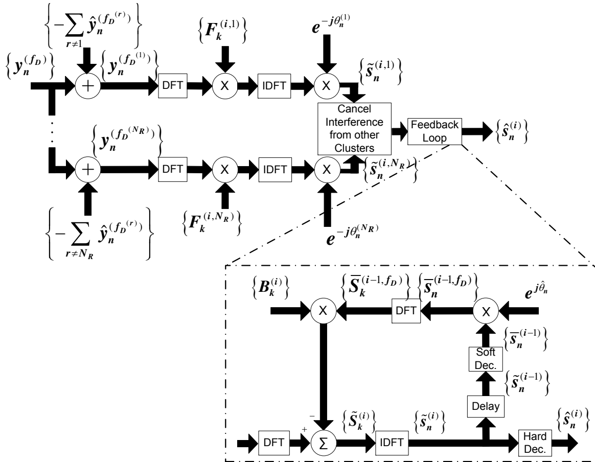
Figure 7.8: Receiver structure for TDC.
