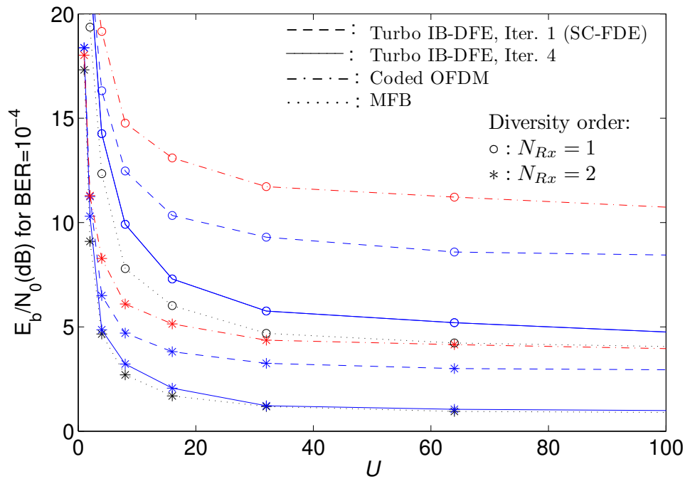
Figure 4.8: Required E_b/N_0 to achieve BER = 10^{-4} for the rate-3/4 convolutional code, as function of the number of multipath components.
