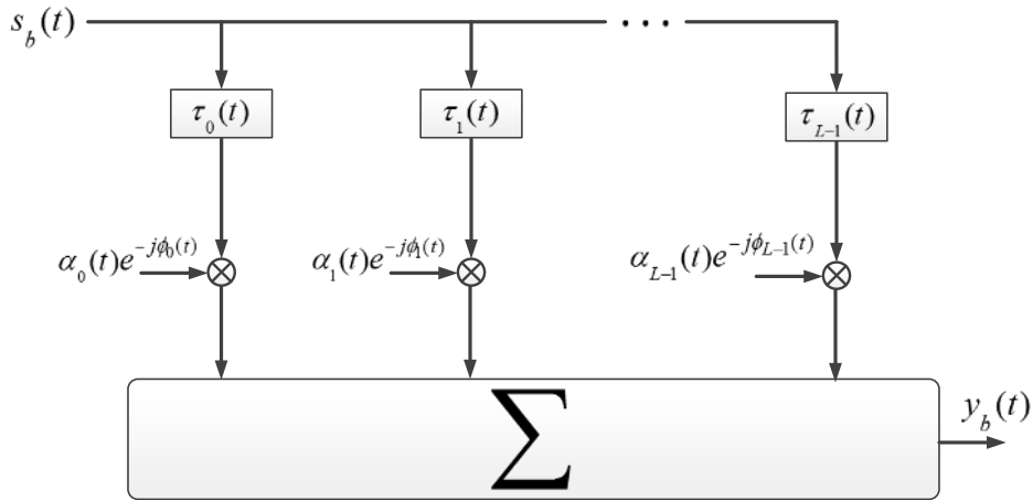
Figure 2.10: Tapped delay line model of a doubly-selective channel in the equivalent complex baseband.
