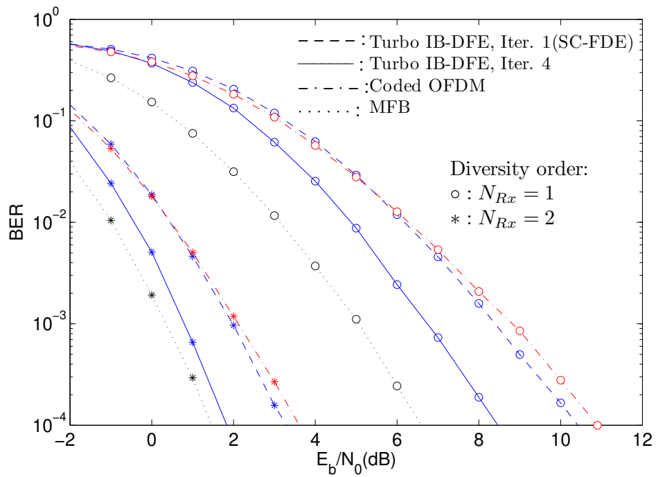
Figure 4.4: BER performance for a rate-2/3 code.
