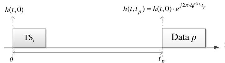
Figure 6.3: Channel estimation for the p th block of data.
