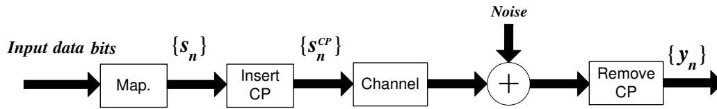
Figure 3.11: Basic SC-FDE transmitter block diagram.
