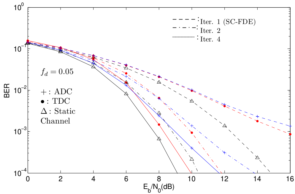
Figure 7.10: BER performance for a scenario with normalized Doppler drifts f_d and -f_d for f_d = 0.05 .
