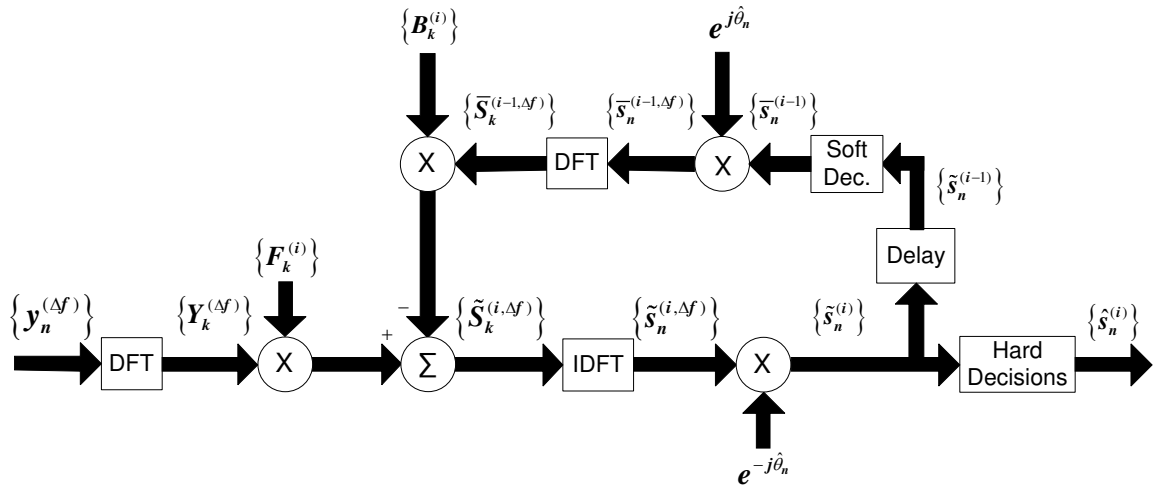
Figure 6.4: Receiver structure for Method II.
