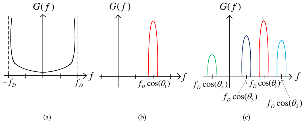
Figure 7.3: Jakes Power Spectral Density (a); PSD associated to the transmission of a single ray (b); PSD associated to the transmission of multiple rays (c).
