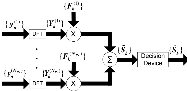
Figure 3.10: OFDM receiver structure with a N_{Rx} -branch space diversity.
