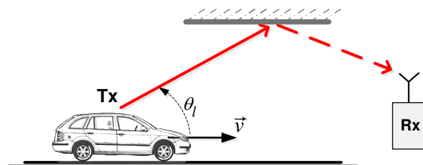
Figure 7.1: Doppler shift.
