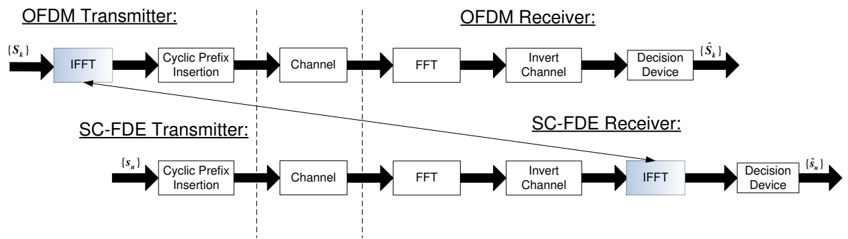
Figure 3.14: Basic transmission chain for OFDM and SC-FDE.
