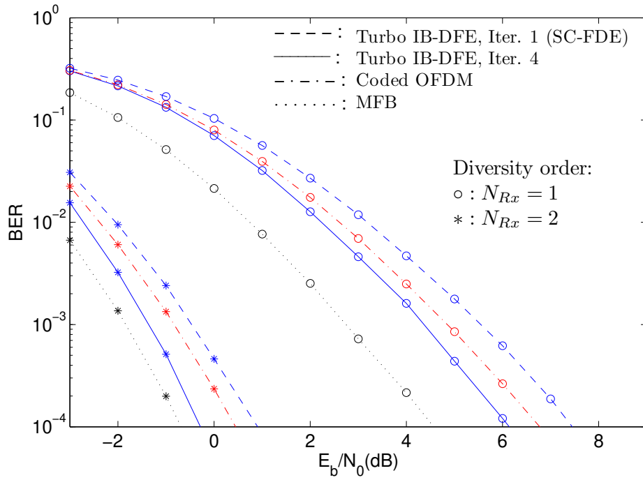
Figure 4.3: BER performance for a rate-1/2 code.
