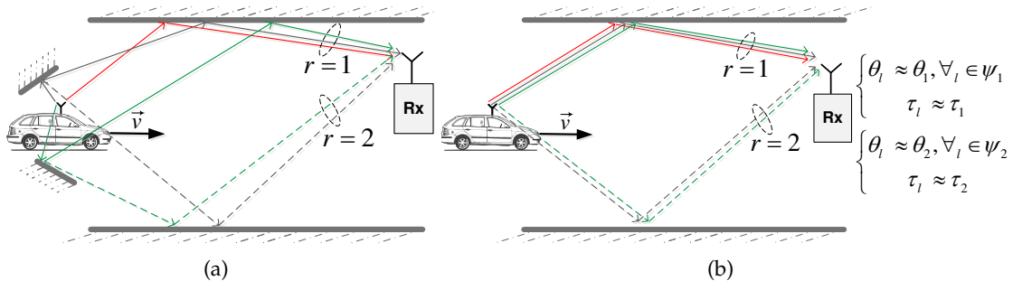
Figure 7.2: Various objects in the environment scatter the radio signal before it arrives at the receiver (a); Model where the elementary components at a given ray have almost the same direction of arrival (b).
