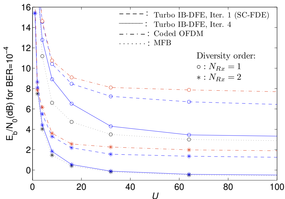
Figure 4.7: Required E_b/N_0 to achieve BER = 10^{-4} for the rate-2/3 convolutional code, as function of the number of multipath components.
