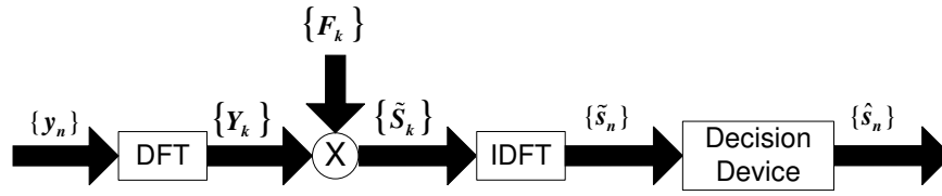
Figure 3.12: Basic SC-FDE receiver block diagram.
