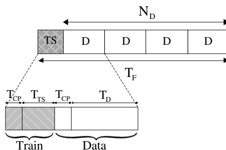
Figure 5.2: Frame structure.
