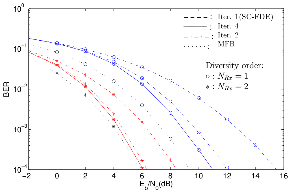
Figure 4.1: BER performance of an IB-DFE in the uncoded case.
