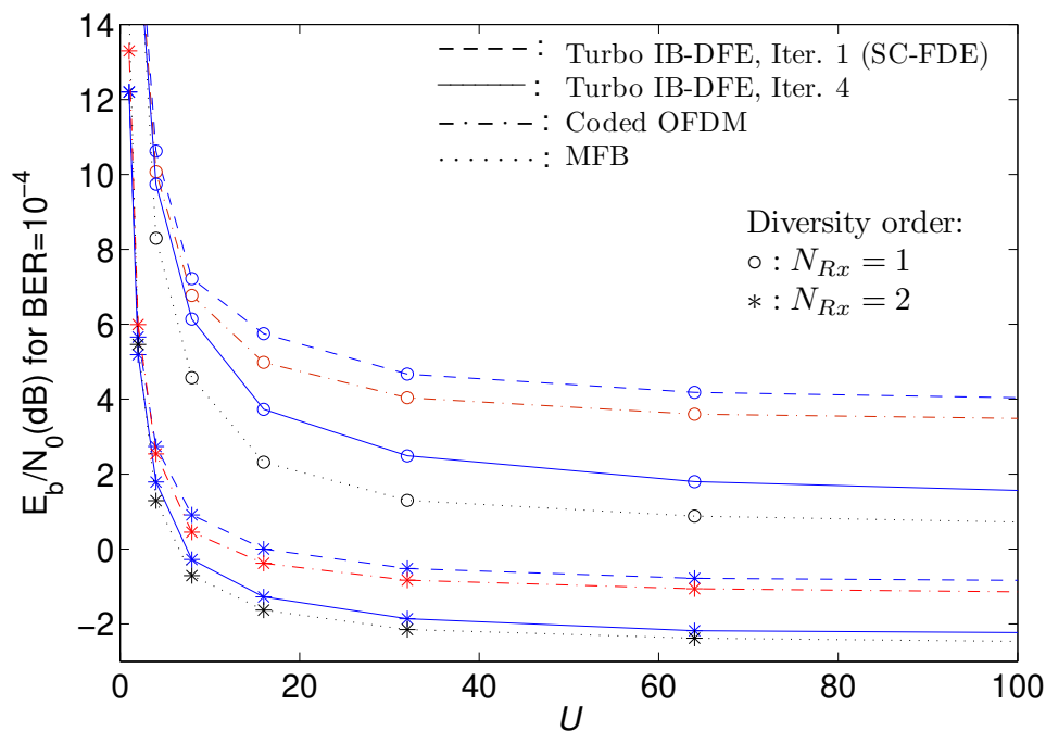
Figure 4.6: Required E_b/N_0 to achieve BER = 10^{-4} for the rate-1/2 convolutional code, as function of the number of multipath components.
