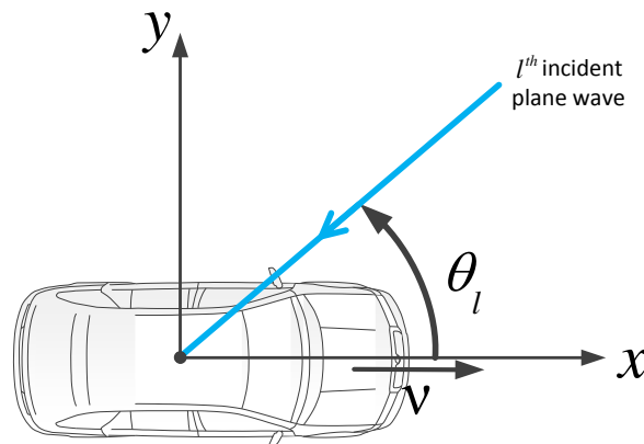
Figure 2.8: Example of a l th incident wave affected by the Doppler effect.
