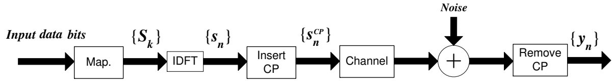
Figure 3.7: Basic OFDM transmission chain.
