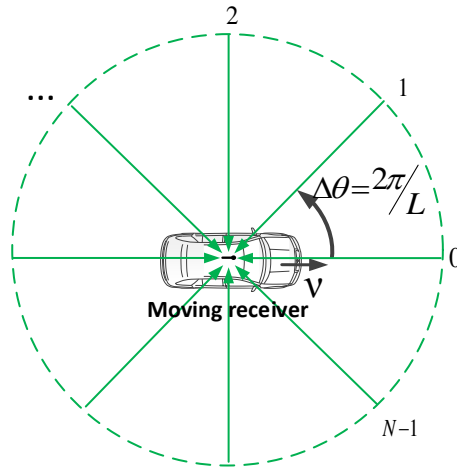
Figure 2.13: Example of an uniform scattering scenario
