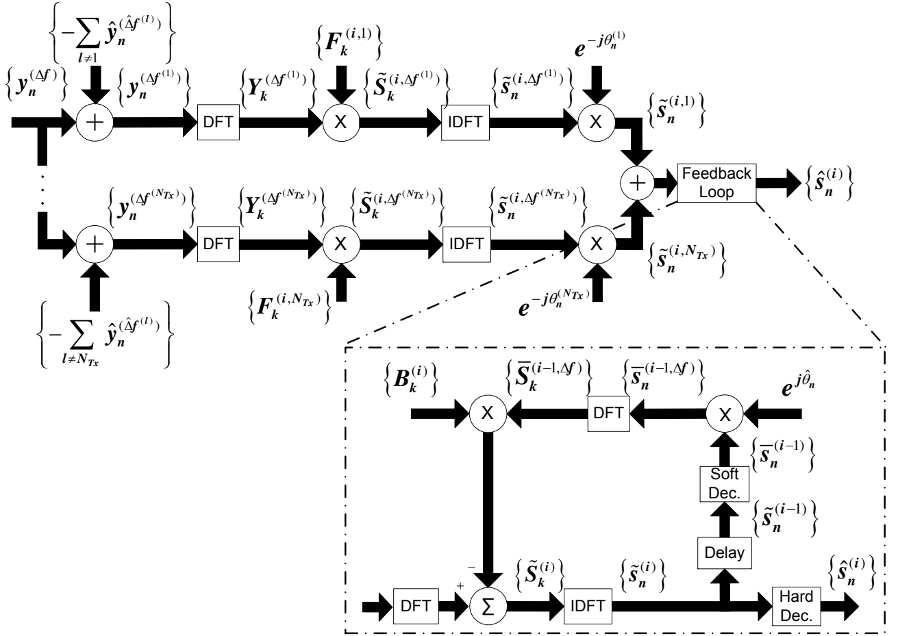
Figure 6.5: Receiver structure for Method III.
