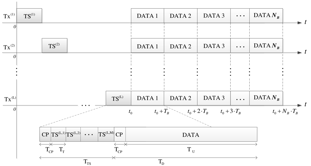
Figure 6.2: Frame structure.
