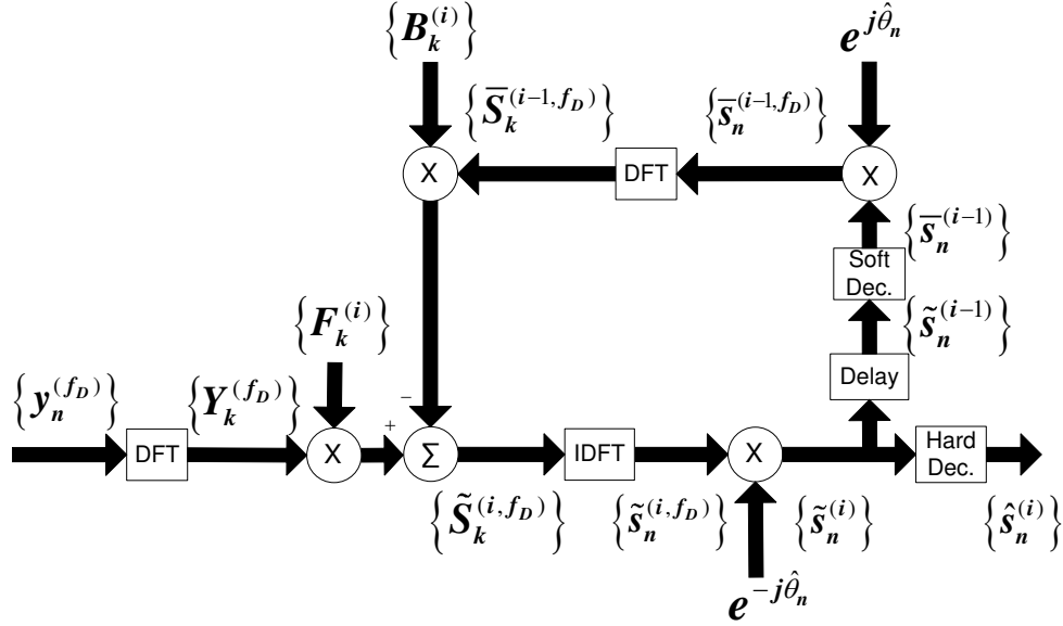
Figure 7.7: Receiver structure for ADC.
