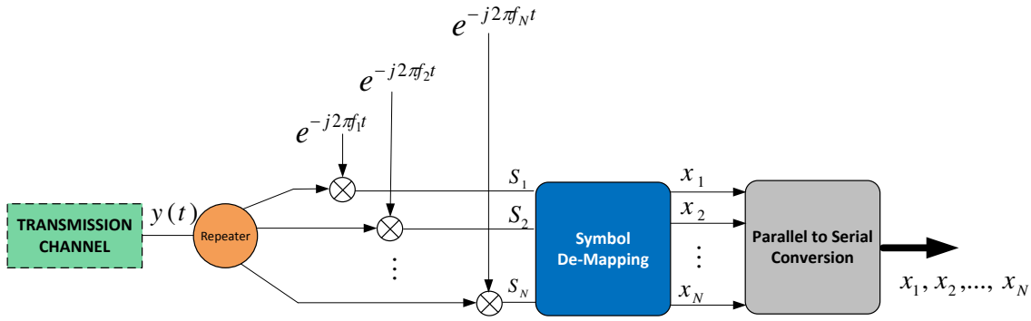
Figure 3.2: Receiving structure for multicarrier modulation.
