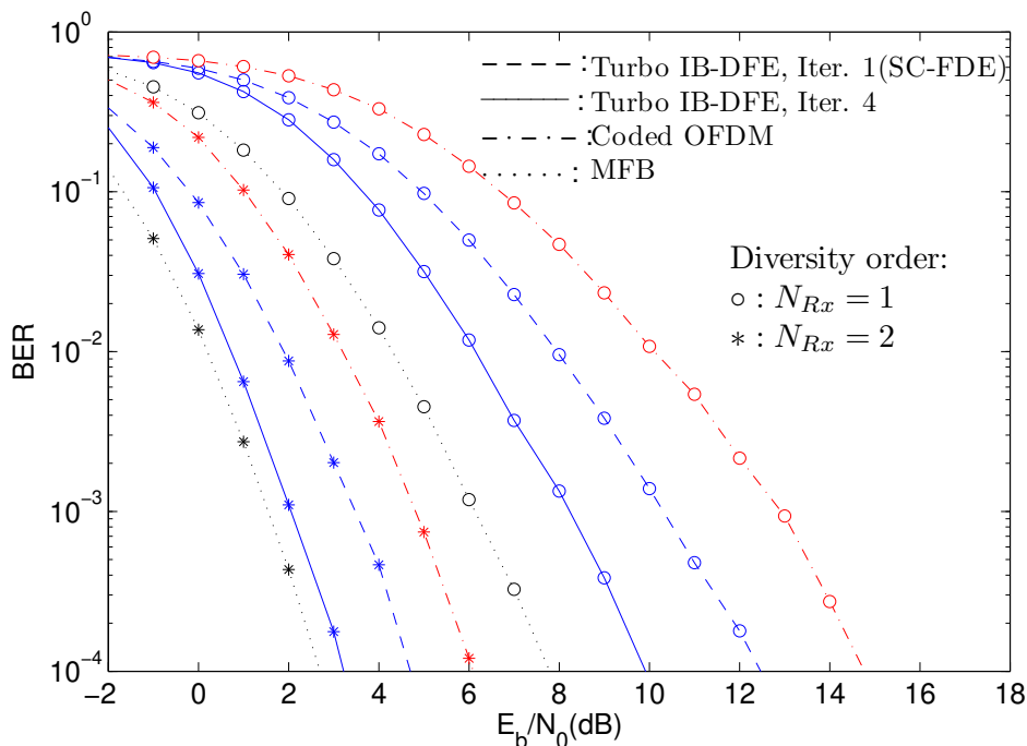
Figure 4.5: BER performance for a rate-3/4 code.
