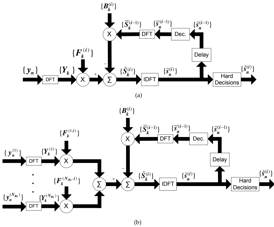
Figure 3.16: IB-DFE receiver structure (a) without diversity (b) with a N_{Rx} -branch space diversity.
