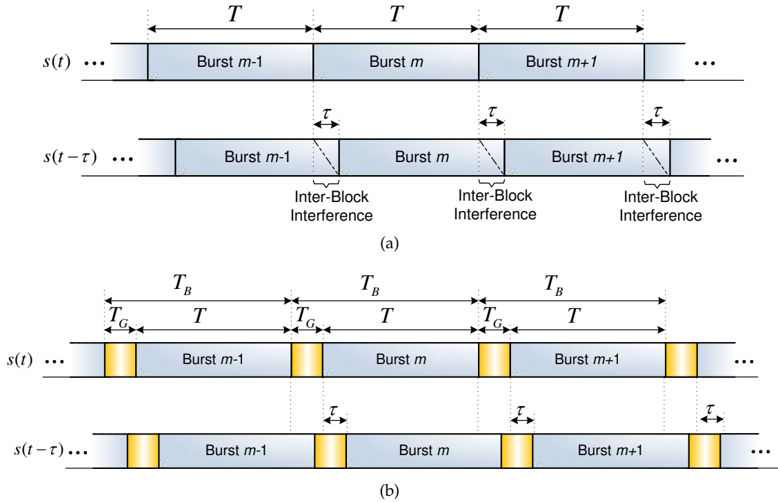
Figure 3.8: (a) Overlapping bursts due to multipath propagation; (b) IBI cancellation by implementing the cyclic prefix.
