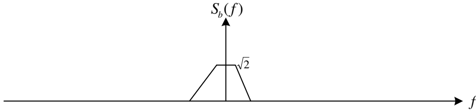
Figure B.3: Equivalent baseband signal spectrum
