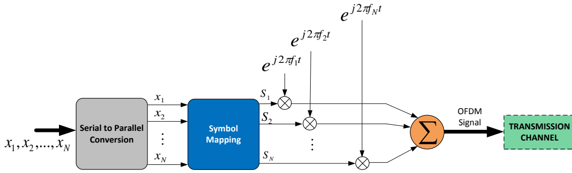
Figure 3.1: Transmission structure for multicarrier modulation.
