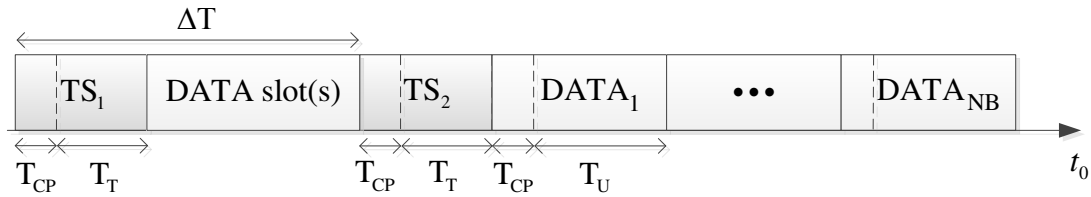
Figure 7.5: Frame structure.
