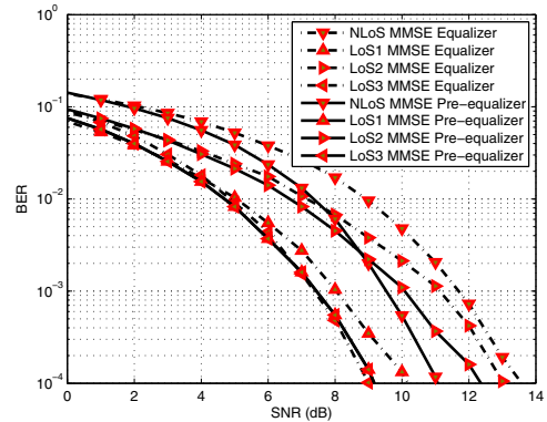
(b) BER Performance under MMSE
