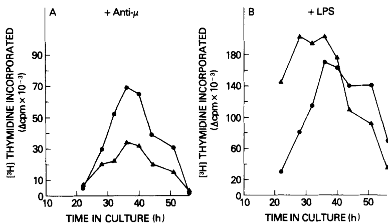
FIG. 2. Time-course of DNA synthesis by density-fractionated B cells stimulated with anti- \mu (A) or LPS (B). B cells at 2 \times 10^5 cells/well in Iscove's/F-12 medium were pulsed with [^3\text{H}] thymidine for 4 h at various times after the addition of anti- \mu or LPS to dense B cells or to intermediate density B cells.
