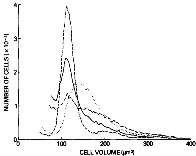
FIG. 1. Cell volume distribution of density-fractionated B cells. Spleen cells from BDF 1 mice were treated with anti-Thy-1.2 and complement and then separated on a Percoll step gradient. Fractions: low density (<1.062), above 50% Percoll; intermediate density (1.062-1.074), 50-60% Percoll; dense (1.074-1.086), 60-70% Percoll. Cell volume was determined by electric resistance and calibrated with microspheres obtained from Coulter Electronics.
