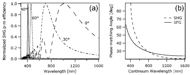
Fig. 1. (a) Normalized SHG phase-matching efficiency of 10- \mu m-thick BBO borate for angles ranging from 0° to 90°; (b) phase-matching angle tuning curve for SHG and SFG with an 800-nm gate pulse.
