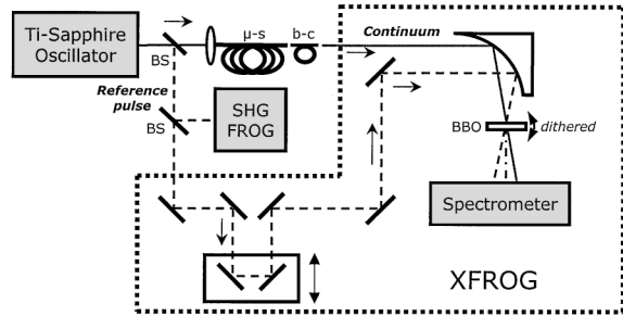
Fig. 2. Schematic diagram of the multishot XFROG measurement apparatus: BSs, beam splitters; \mu -s, microstructure fiber; b-c, butt-coupling fiber.
