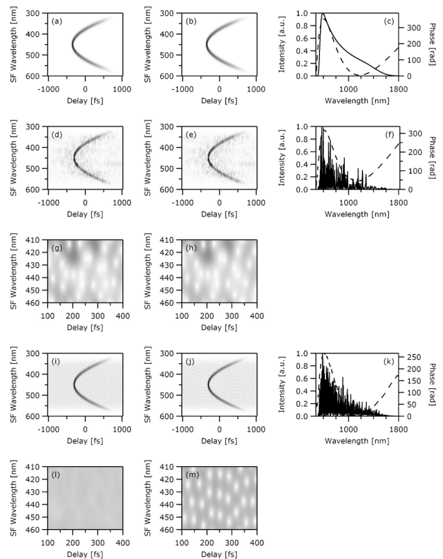
Fig. 5. Simulations: (a) theoretically generated and (b) retrieved XFROG traces. (c) Retrieved spectral intensity and phase of a pulse of a smooth super-Gaussian spectrum and cubic spectral phase; XFROG error, 0.00015. (d) Theoretically generated and (e) retrieved XFROG traces. (f) Retrieved spectral intensity and phase of a pulse with a structured XFROG error, 0.00031. (i) Average of 100 such structured traces. (j) Retrieved XFROG trace and (k) retrieved spectral intensity and phase from (i); XFROG error, 0.0027. (g), (h), (l), and (m) are higher-resolution sections in (d), (e), (i), and (j), respectively. All the traces are 1024 \times 1024 in dimension. SF, sum frequency.
