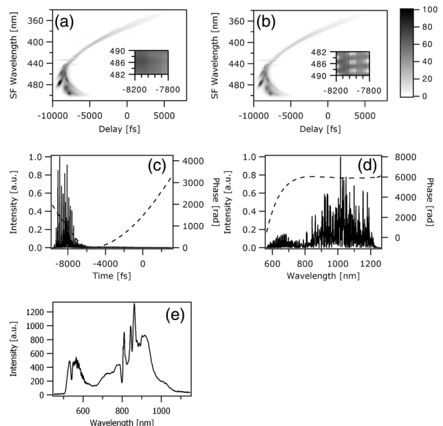
Fig. 3. XFROG measurement of the microstructure-fiber continuum with an 800-nm 30-fs precharacterized reference pulse: (a) measured trace, (b) retrieved trace, (c) retrieved temporal intensity (solid curve) and phase (dashed curve), (d) retrieved spectral intensity (solid curve) and phase (dashed curve), (e) independently measured spectrum. The XFROG error was 0.012. The insets in (a) and (b) are higher-resolution sections in the traces. Both traces are 8192 \times 8192 in dimension. SF, sum frequency.
