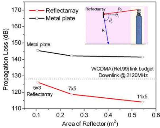
Fig. 18. Link budget analysis of propagation gain in WCDMA (Rel. 99) system using various reflectors.
