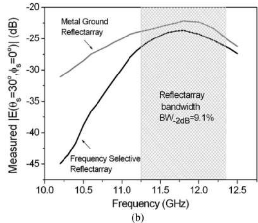
Fig. 10. (a) Experimental models of FSR and conventional metal ground reflectarray. (b) Comparison of measured electrical field magnitude of the two reflectarrays in the direction of the main beam.
