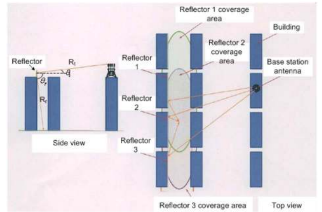
Fig. 14. Elimination of blindness using reflectarrays in wireless communication system.
