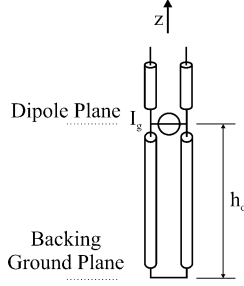
Fig. 10. Generic transmission line model for a Floquet mode in presence of the connected dipole array backed with a ground plane. The transmission line model is the same for TE and TM modes once the proper definition of the characteristic line impedance is chosen. I_g is a unit current generator.
