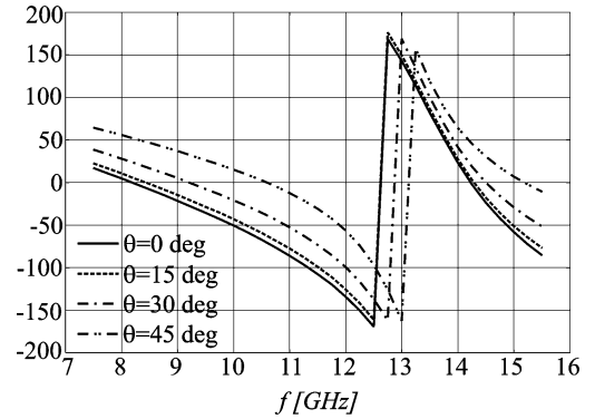
Fig. 4. Phase of the reflection coefficient of the FSS backed by a ground plane for different angles of incidence for TE-polarized plane wave incidence.
