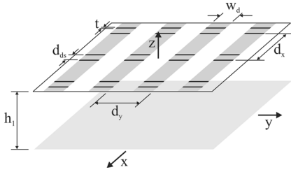
Fig. 1. 3-D view of the antenna structure with ground plane.
