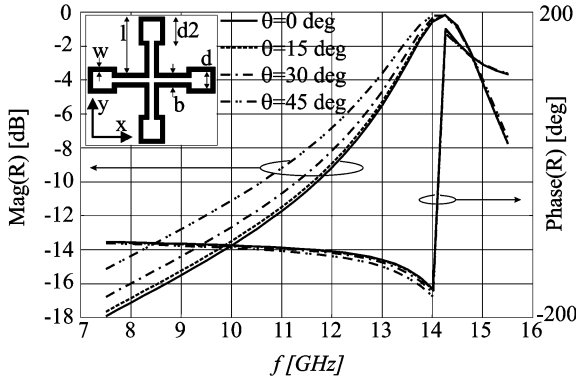
Fig. 3. Magnitude and phase of the reflection coefficient of the FSS for different angles of incidence for TE-polarized plane wave incidence.
