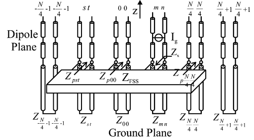
Fig. 12. Equivalent transmission line model of the planar structure of Fig. 9.
