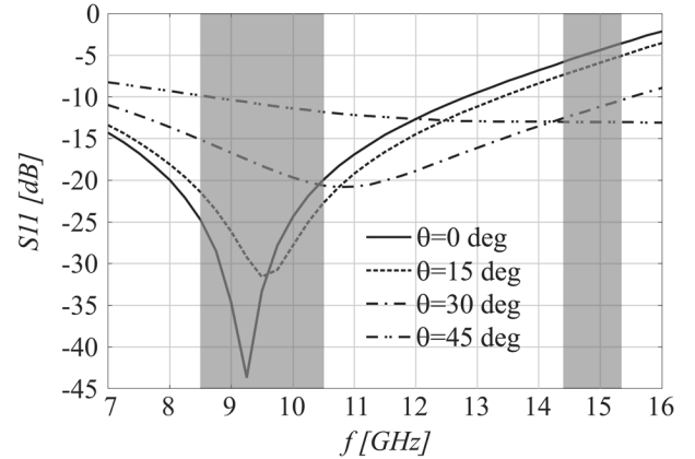
Fig. 2. Magnitude of the active reflection coefficient of the connected dipole array antenna with the ground plane. Gray strips indicate the considered operative bands.
