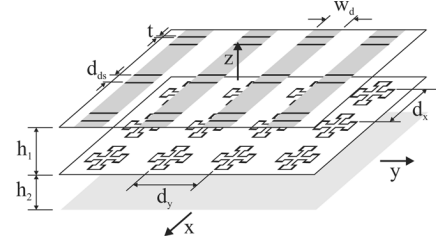
Fig. 9. 3-D view of the antenna structure with the FSS and the ground plane.
