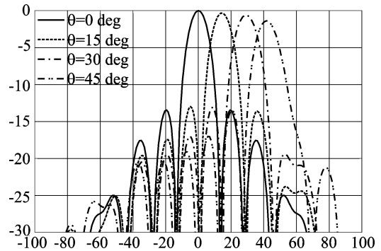
Fig. 15. Radiation patterns on the H-Plane for different scan angles at the central frequency of the TCDL band, f = 15 GHz, for the connected dipole array antenna backed by the ground plane and FSS. The pattern are normalized to the maximum value for broadside radiation.
