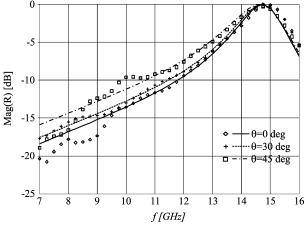
Fig. 7. Measured magnitude of the reflection coefficient of the FSS for different angles of incidence for TE-polarized plane wave incidence. Lines refer to HFSS results while symbols to measurement.
