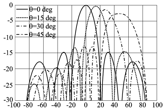
Fig. 14. Radiation patterns on the H-Plane for different scan angles at the central frequency of the radar band, f = 9.5 GHz, for the connected dipole array antenna backed by the ground plane and FSS. The pattern are normalized to the maximum value for broadside radiation.
