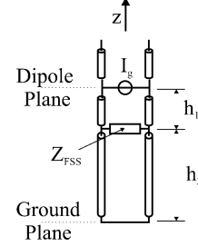
Fig. 11. Equivalent transmission line model of the planar structure of Fig. 9 for the main FW's mode. h_1 and h_2 are respectively the distance of the FSS from the connected dipole array and from the backing ground plane.
