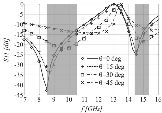
Fig. 13. Magnitude of the active reflection coefficient of the connected dipole array antenna with the FSS and the ground plane. Lines refer to HFSS results while symbols to the in-house method.
