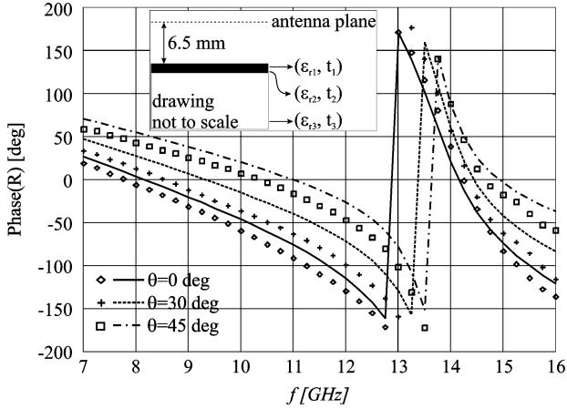
Fig. 8. Measured phase of the reflection coefficient of the FSS backed by a ground plane for different angles of incidence for TE-polarized plane wave incidence. Lines refer to HFSS results while symbols to measurement.
