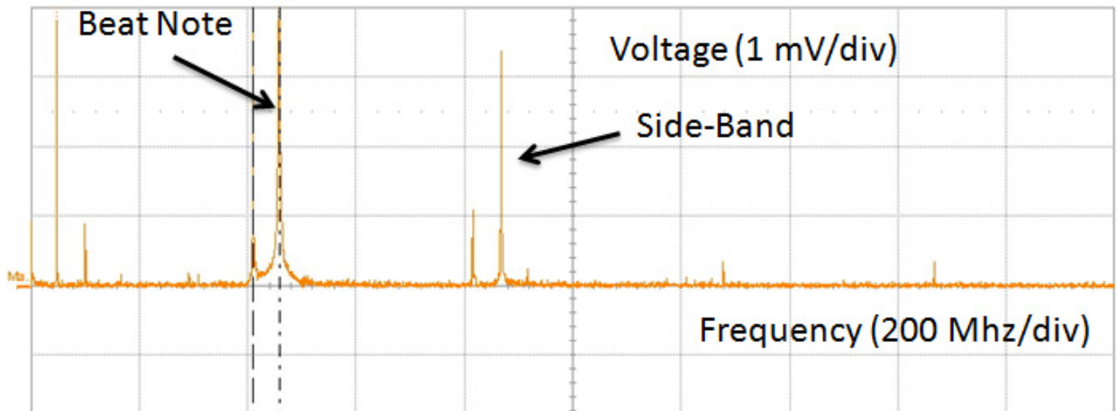
Figure 24: The beat note frequency can be seen above along with the sidebands associated with it (one sideband on either side of the beat note).
