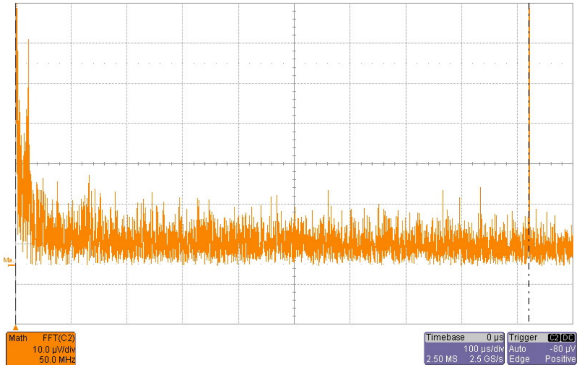
Figure 26: Beat frequency measurement with the diode laser in mode-locking. Several large signals are seen in the low RF range and the 460 MHz signal can be seen.
