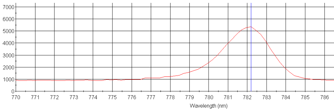
Figure 12: Spectrum of the mode-locked diode laser at 460 MHz and -7 dBm
