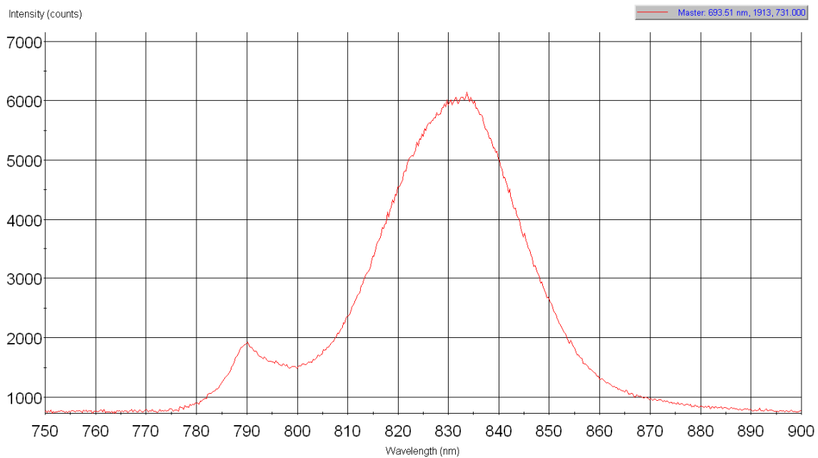
Figure 17: Spectrum of the femtosecond Ti:Sapph laser showing little signal over the 784 nm range and multiple modes.
