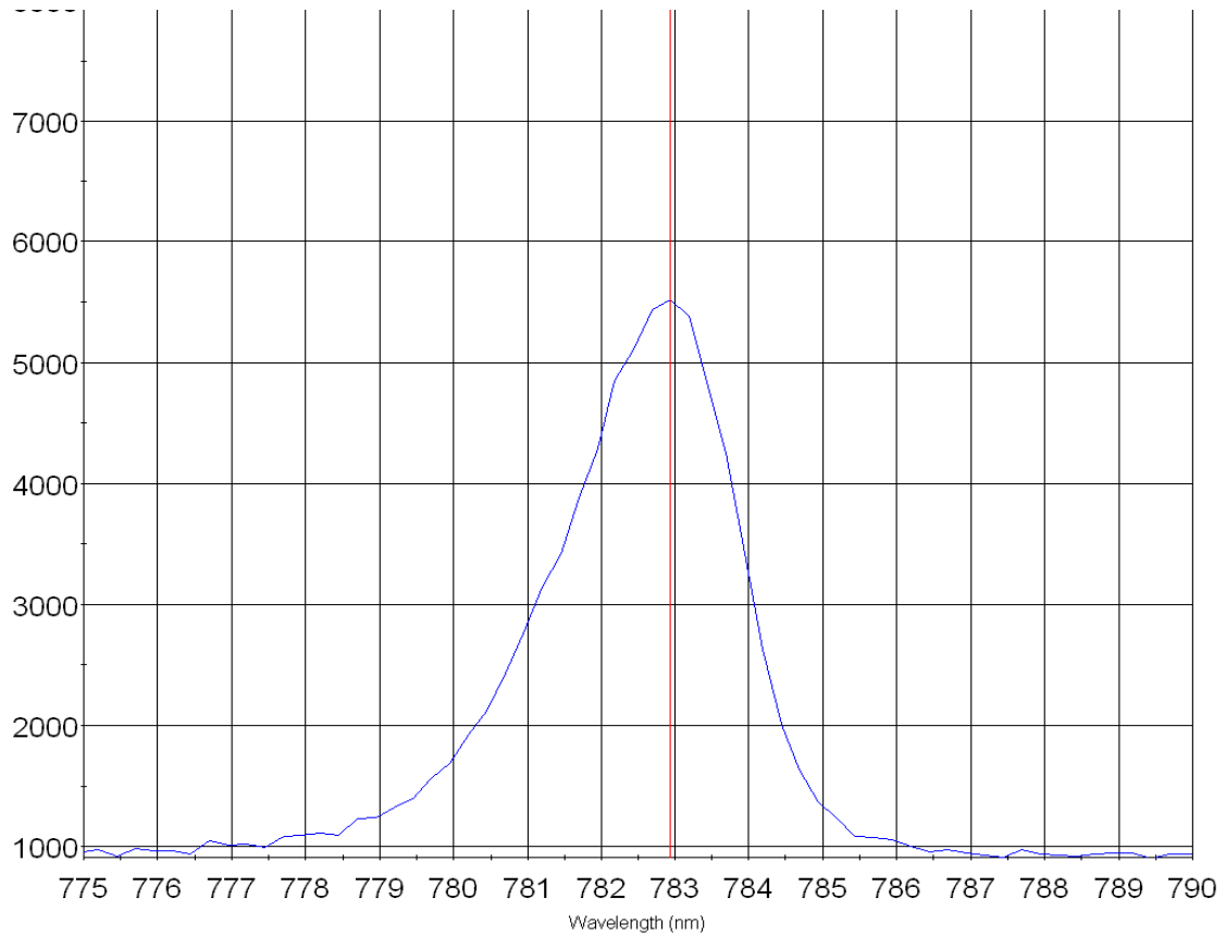
Figure 30: Spectrum of the mode-locked diode laser with the 780 nm optical bandpass filter in the laser cavity. The intensity of the spectrum, bandwidth, centerline, and general shape all appear to have changed.
