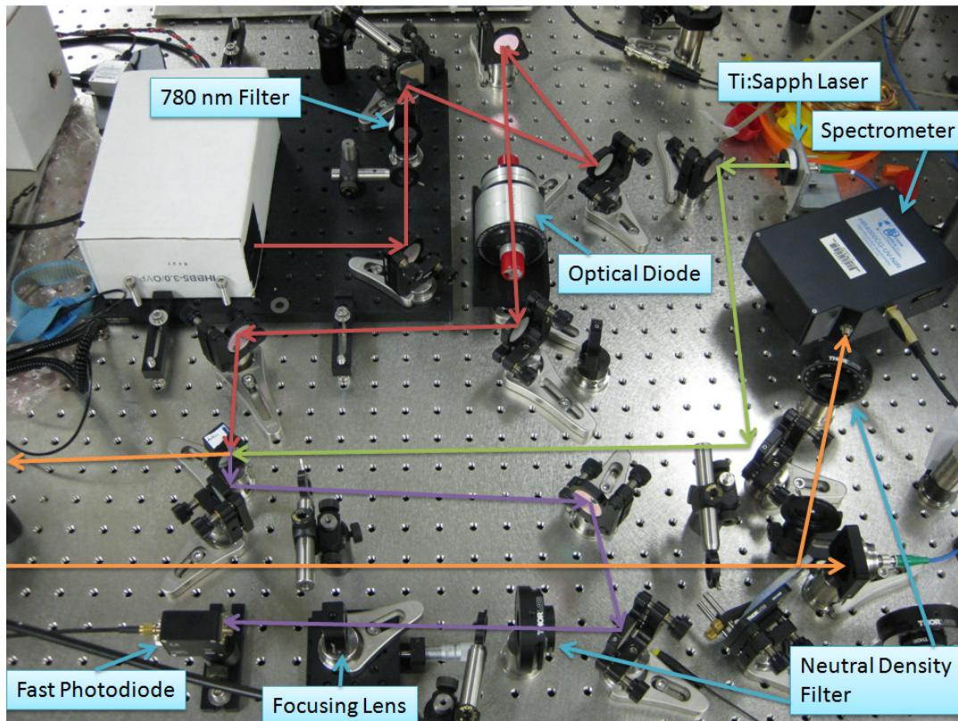
Figure 18: Setup for the beat note frequency experiment using the mode-locked diode laser. The diode laser is shown in red. The Ti:Sapph is shown in green. The combined beam sent to the spectrometer and fiber coupler is shown in orange. The combined beam sent to the photodiode is shown in purple.
