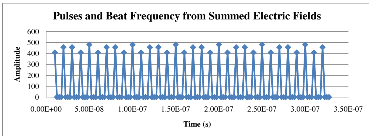
Figure 9: Pulses and Beat Frequency from summation of electric fields.
