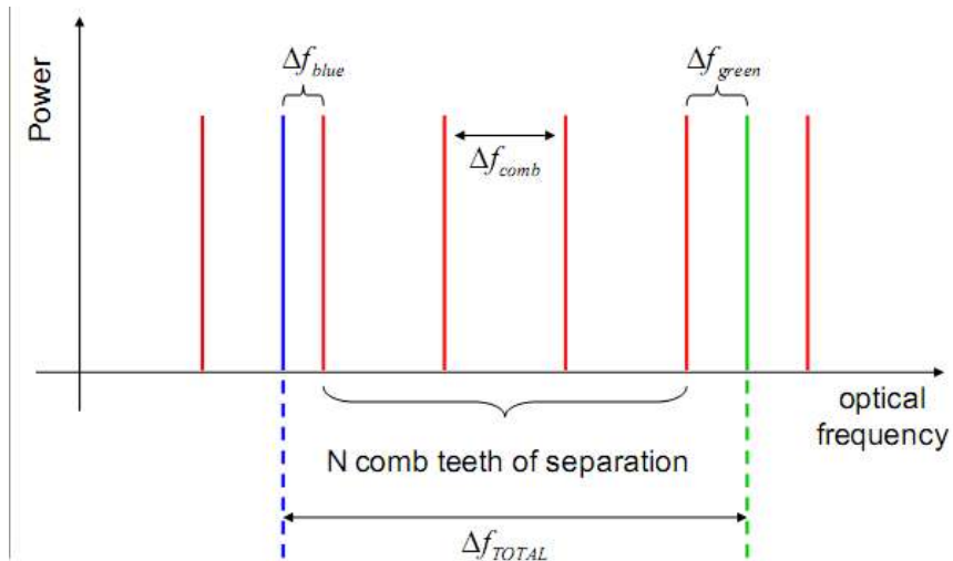
Figure 2: The even spacing of the comb teeth as well as the separation between two lasers can be seen. The green and blue lasers represent two continuous wave lasers being compared using the optical frequency comb.
