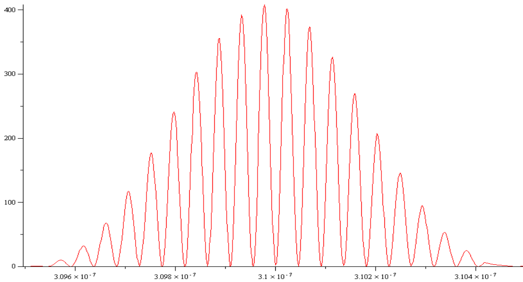
Figure 8: Single pulse of the overlapping electric fields as simulated by Maple.
