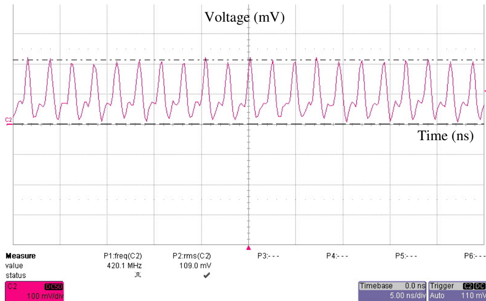
Figure 6: Pulsed output of a diode laser in active mode-locking.
