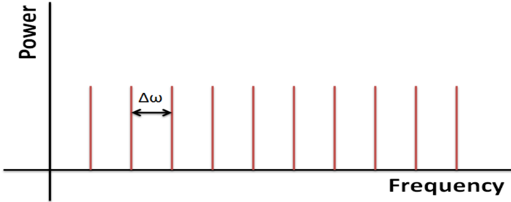
Figure 1: Evenly spaced Dirac delta functions create a comb-like structure in frequency space that can act as a frequency ruler.
