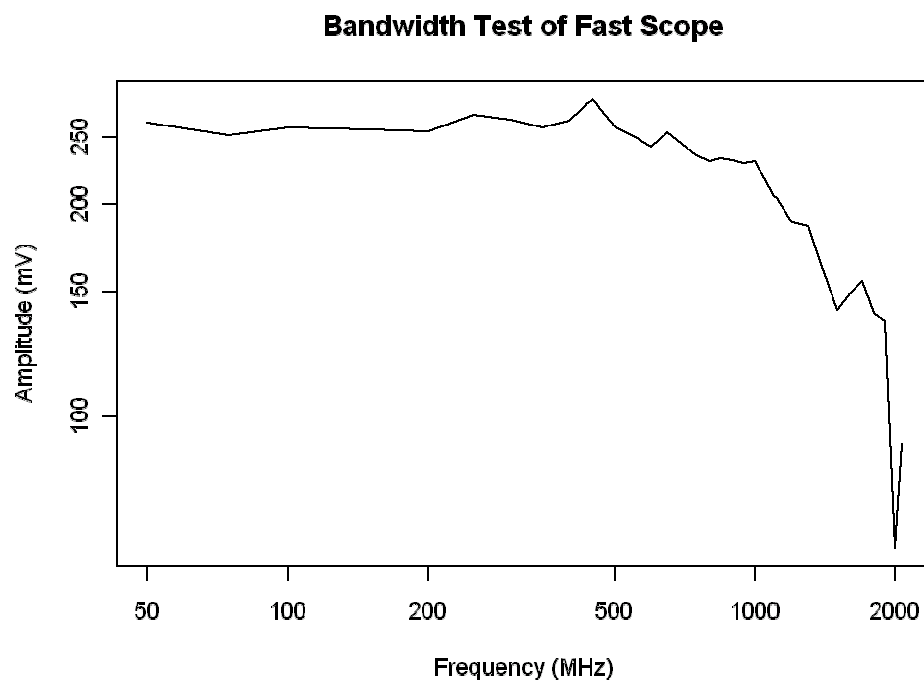
Figure 32: Bandwidth test of the 1 GHz oscilloscope. Shows a sharp drop off after 1 GHz and a mostly stable signal before 1 GHz.
