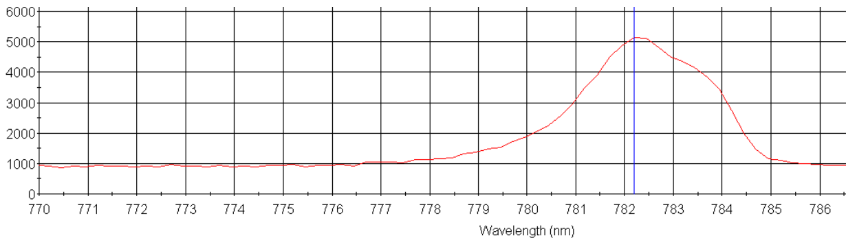
Figure 13: Spectrum of the mode-locked diode laser at 420 MHz displaying the possible existence of multiple modes. This was observed by opening the iris within the laser cavity which may have led to a partial hybrid passive and active mode-locking system
