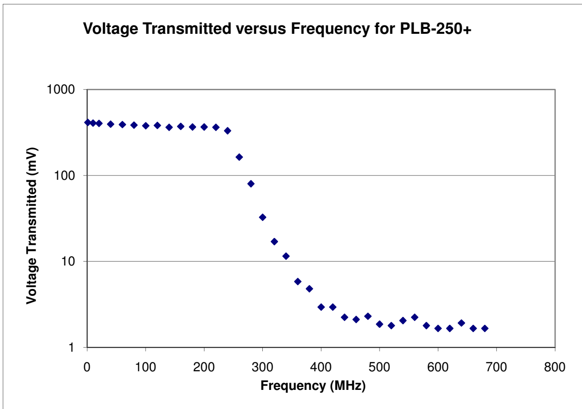
Figure 21: Characterization of the PLB-250+ low-pass filter showing a sharp cutoff at 260 MHz and a reduction of a factor of 200 in the signal of higher frequencies.
