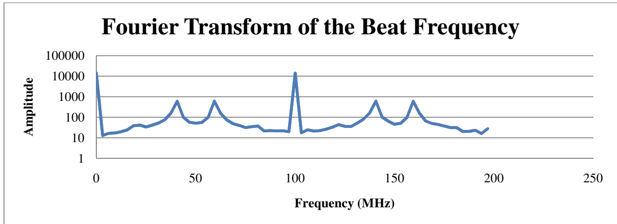
Figure 10: Fourier transform of the beat frequency data. A large peak is seen at both the DC point and the 100 MHz point. The 100 MHz peak corresponds to the beat note between the peaks of the optical frequency comb. The peaks at 40 and 60 MHz are the beat frequency peaks of the continuous wave laser and the nearest comb. The 140 and 160 MHz terms are the beat frequency peaks of the continuous wave laser and the next nearest comb.
