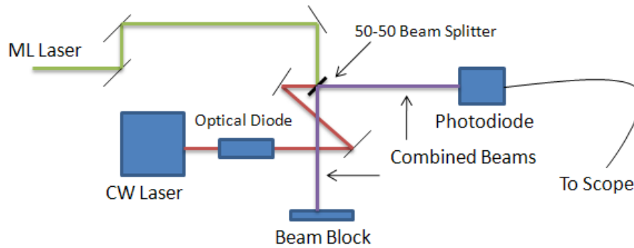
Figure 16: Setup for the beat frequency measurement using the femtosecond mode-locked Ti:Sapph laser.
