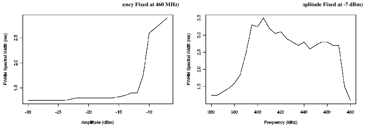
Figure 14: Amplitude Optimization of Mode-Locked Diode Laser Spectrum (Left) Frequency Optimization of Mode-Locked Laser Spectrum (Right)
