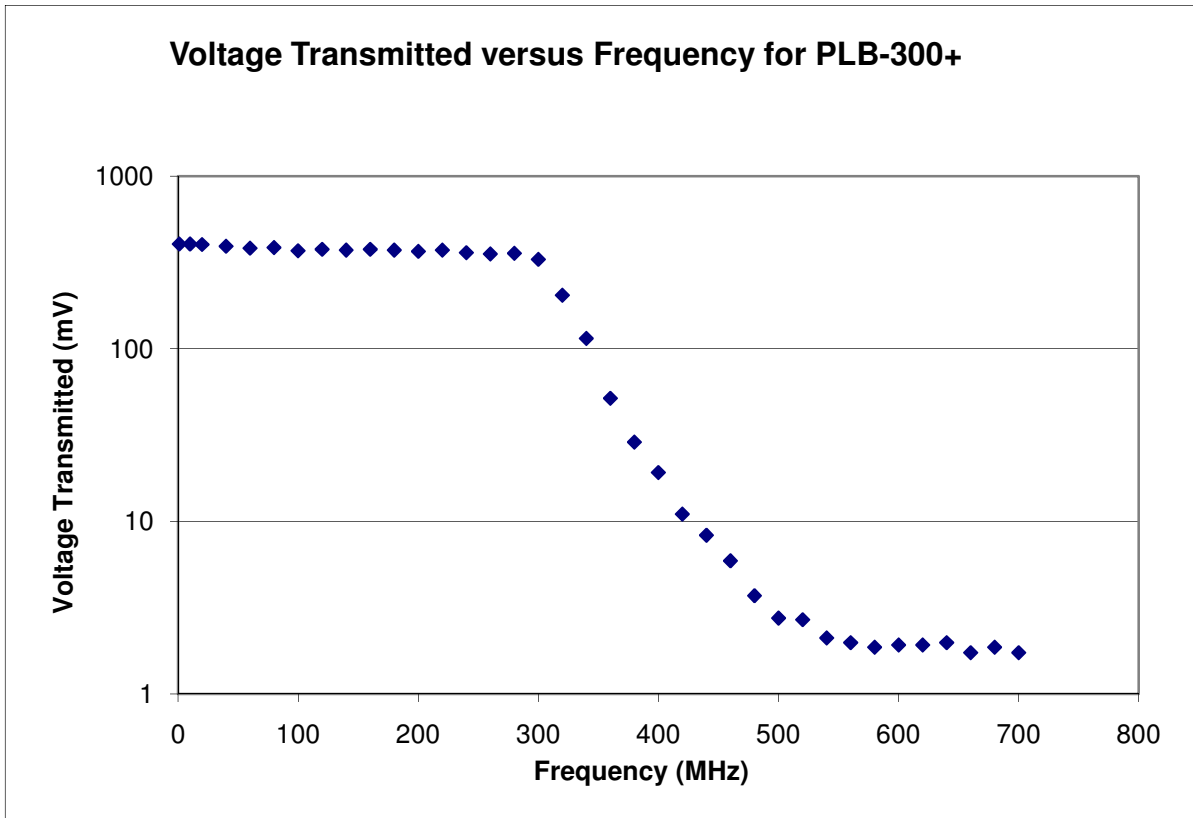
Figure 22: The characterization of the PLB-300+ low-pass filter showing a sharp cutoff at 300 MHz and a reduction of a factor of 200 in the higher frequencies.
