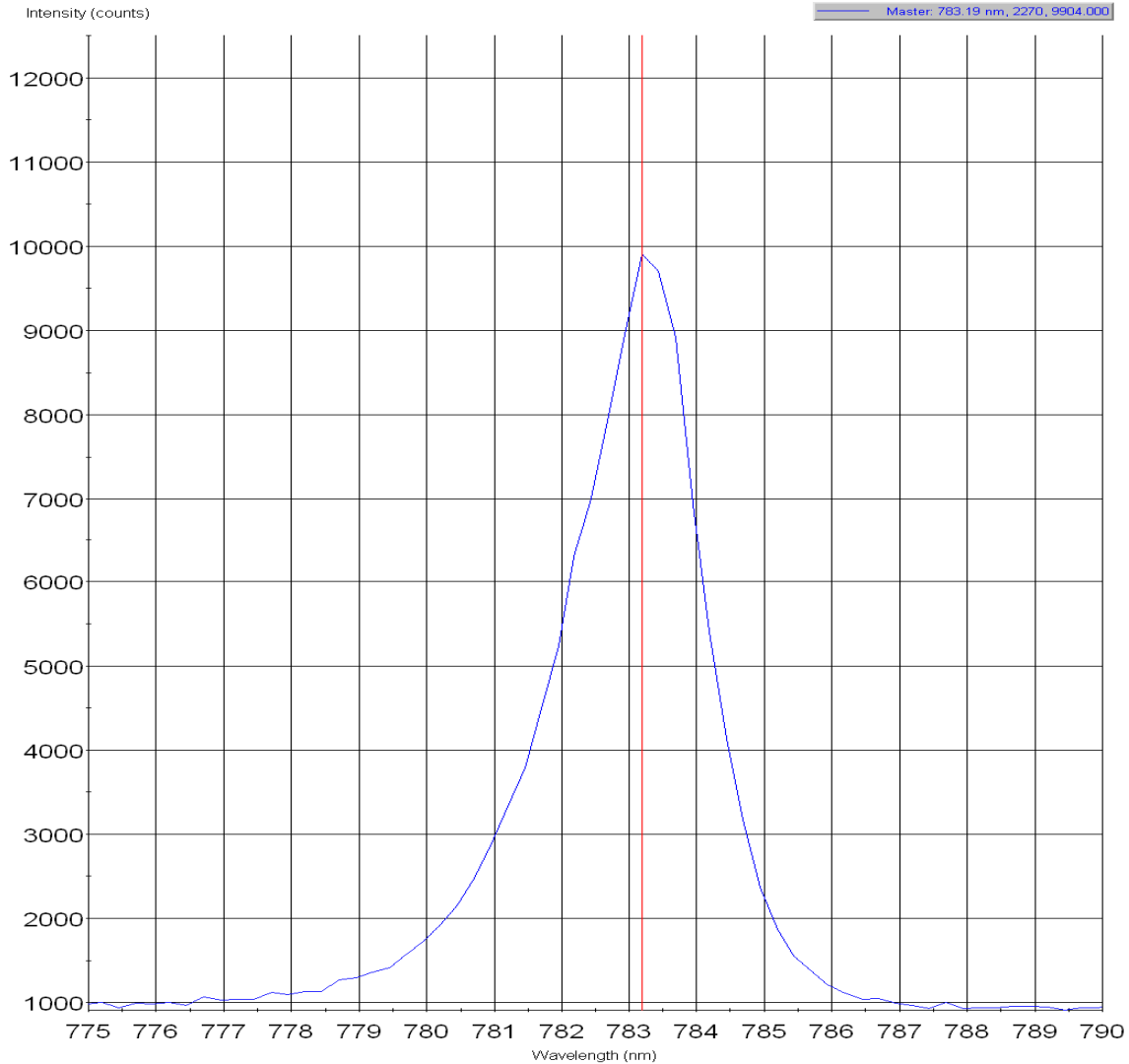
Figure 31: Spectrum of the mode-locked diode laser with a piece of glass placed inside the laser cavity in place of the optical band pass filter.
