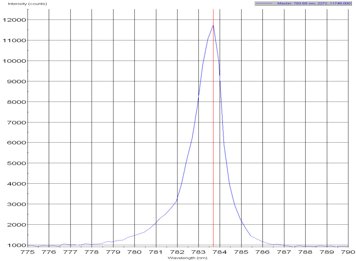
Figure 29: Spectrum of the mode-locked diode laser without any filters within the laser cavity
