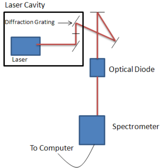
Figure 11: Setup to record the spectrum of the mode-locked diode laser
