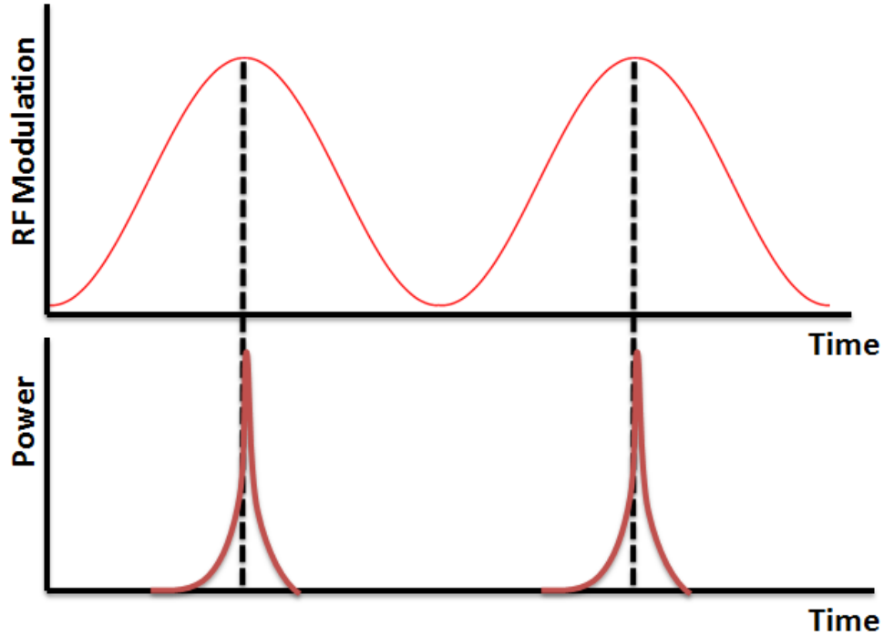
Figure 4: This shows the RF modulation and power of the diode laser as a function of time. The maximum of the RF modulation falls when the laser signal returns to the gain medium and gets amplified. Over time this will lead to a pulsed output as the pulses will continue to be amplified while everything else will eventually fade out.
