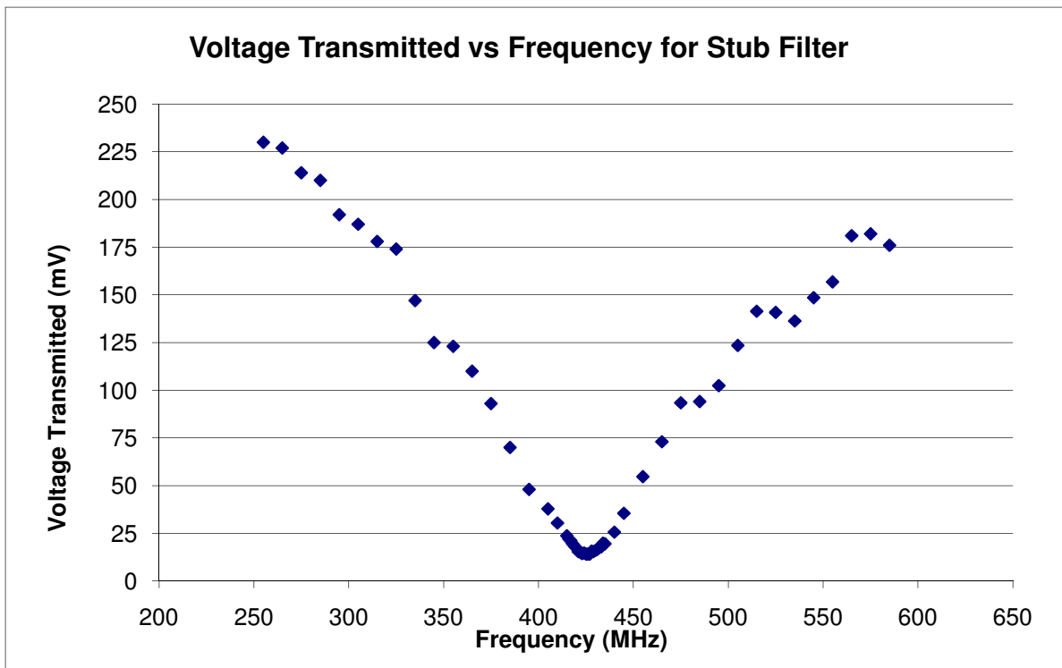
Figure 20: The characterization of the stub filter showing that the target frequency was reduced by a factor of 16 but that it does not prevent higher harmonics from coming through.
