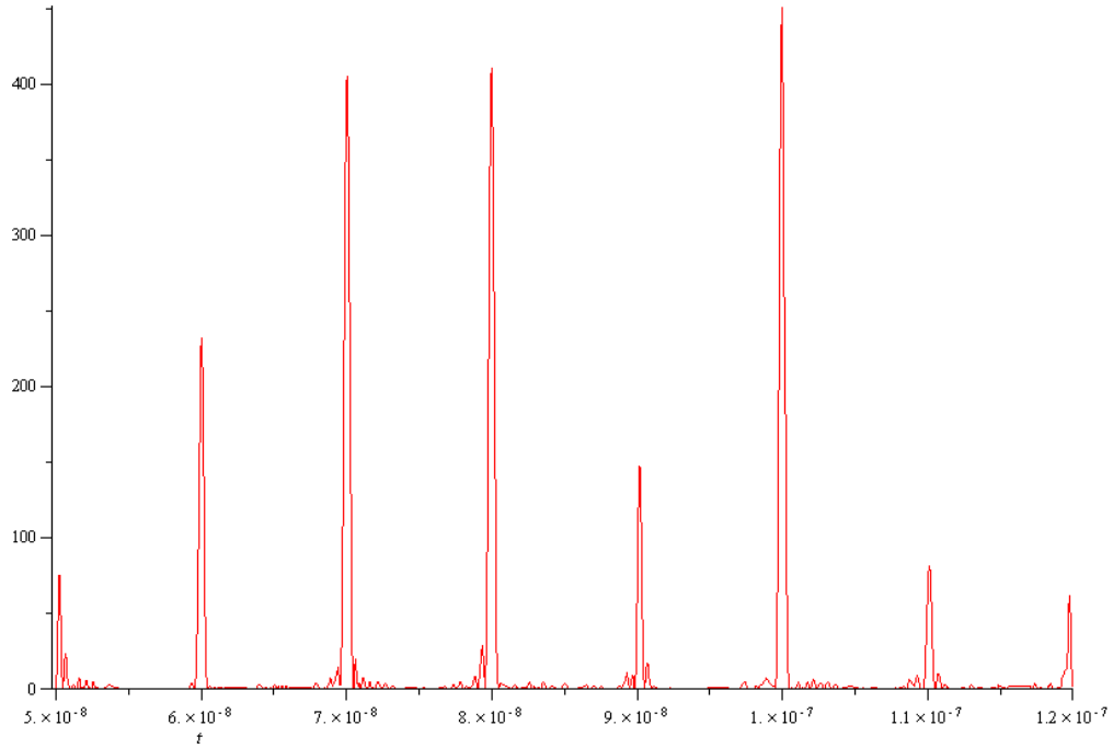
Figure 7: Simulated mode-locked laser in the time domain with the added continuous wave laser.
