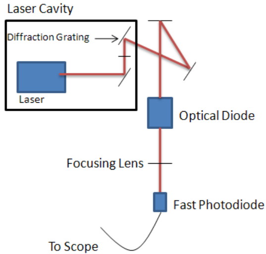
Figure 5: Setup used to verify active mode-locking
