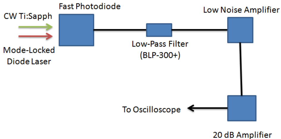
Figure 23: Circuit diagram for the filter and amplifiers.
