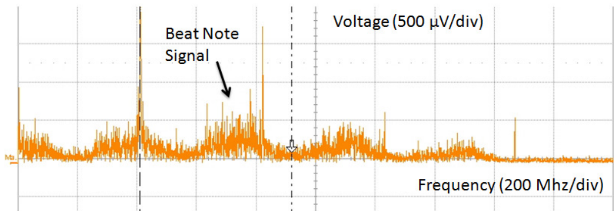
Figure 25: Noisy beat note signal seen as the amplitude of the RF signal was increased. This showed that there may have been some partial mode-locking occurring at the low amplitudes.
