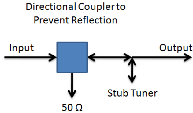
Figure 19: Setup for the stub filter. The path labeled “Stub Tuner” was the path set to \frac{1}{4} the wavelength of the target frequency and was left without termination. A directional coupler was used to prevent reflections from returning to the source.
