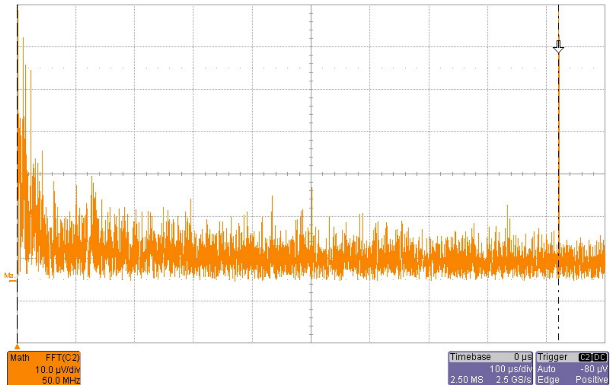
Figure 28: Frequency space representation of the overlapped laser beams showing no beat note frequency with the 780 nm optical bandpass filter added to the laser cavity.
