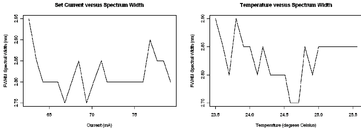
Figure 15: Set Current Optimization of Mode-Locked Diode Laser Spectrum (Left) Temperature Optimization of Mode-Locked Diode Laser Spectrum (Right)
