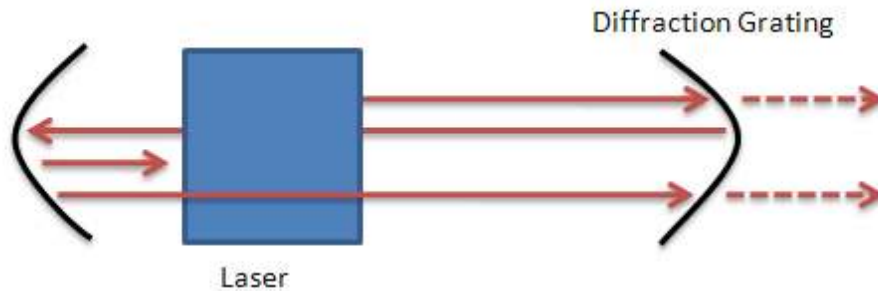
Figure 3: Schematic for the cavity of a diode laser. The blue square is the gain medium used to create the laser. In the case of a diode laser making use of passive mode-locking, the diffraction grating would be replaced with a saturable absorber. The diffraction grating would be used in the case of a diode laser in active mode-locking.
