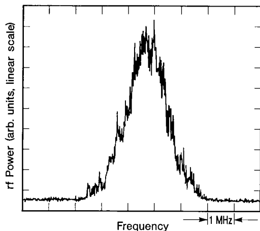
Fig. 3. Heterodyne beat spectrum between the fiber laser and the He-Ne laser averaged over twenty 50-msec samples with a 100-kHz resolution bandwidth. The beat spectrum is centered at 468 MHz and has a FWHM of 1.6 MHz.
