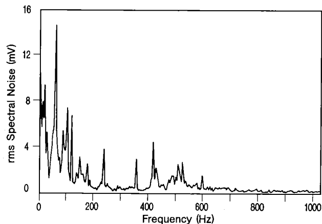
Fig. 2. Spectrum of the frequency fluctuations of the free-running fiber laser using the side of the FP spectrum analyzer transmission peak as a frequency discriminant. A 10-mV change in transmission through the FP spectrum analyzer corresponded to a laser frequency change of approximately 200 kHz.
