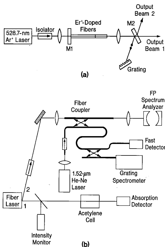
Fig. 1. (a) Schematic diagram of the Er-doped fiber laser. (b) Diagram of the apparatus for measuring the beat spectrum between the fiber laser and the 1.523- \mu\text{m} He-Ne laser and for detecting absorption lines of acetylene. The second fiber coupler operates as a beam splitter for the mixed signal.
