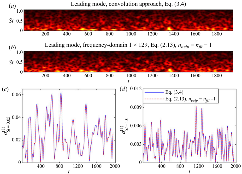
Figure 24. Comparison between two strategies for SPOD-based frequency–time analysis: frequency–time diagrams for (a) the convolution approach (SPOD modes precomputed with 50% overlap) and (b) the frequency-domain approach using n_{ovlp} = n_{fft} - 1 ; expansion coefficients for (c) St = 0.05 and (d) St = 1.0 .
