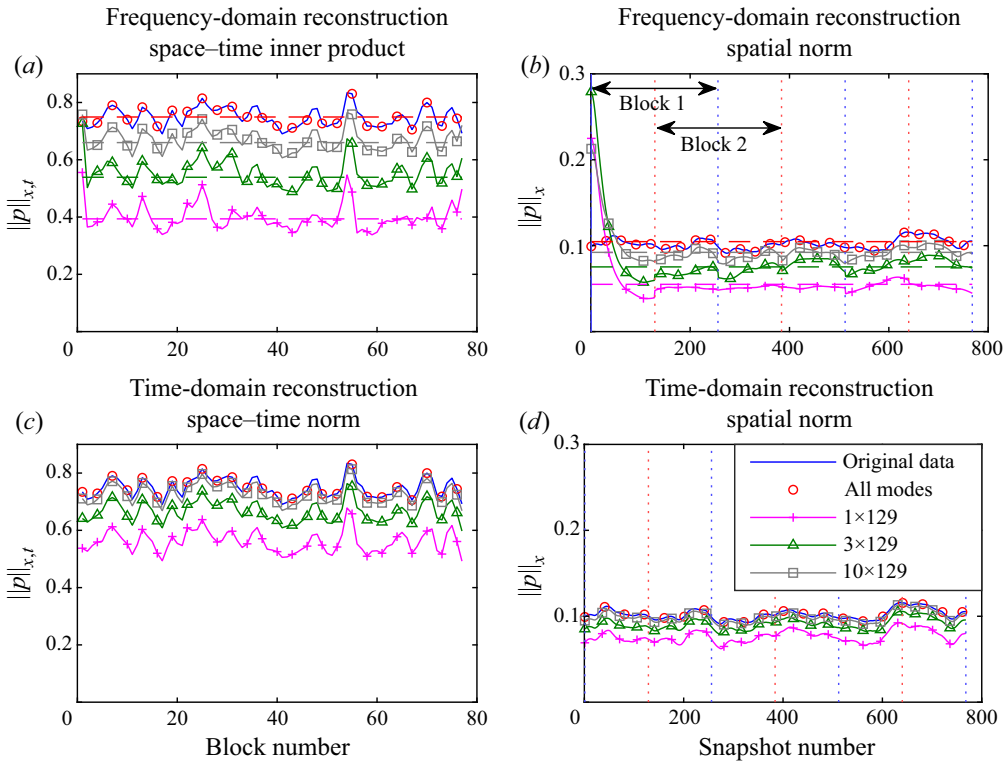
Figure 4. Low-dimensional reconstruction of the jet data: frequency-domain reconstruction ( a,b ), and time-domain reconstruction ( c,d ) in terms of the space-time norm ( a,c ) and the spatial norm ( b,d ). The original data (blue lines), shown for reference, are compared with the full reconstructions using all modes, and reconstructions using 10 \times 129 , 3 \times 129 and 1 \times 129 modes. Summed SPOD mode energies are shown as dashed lines. Vertical dotted blue and red lines in ( b,d ) indicate the left and right blocks in the reconstruction (see figure 1).
