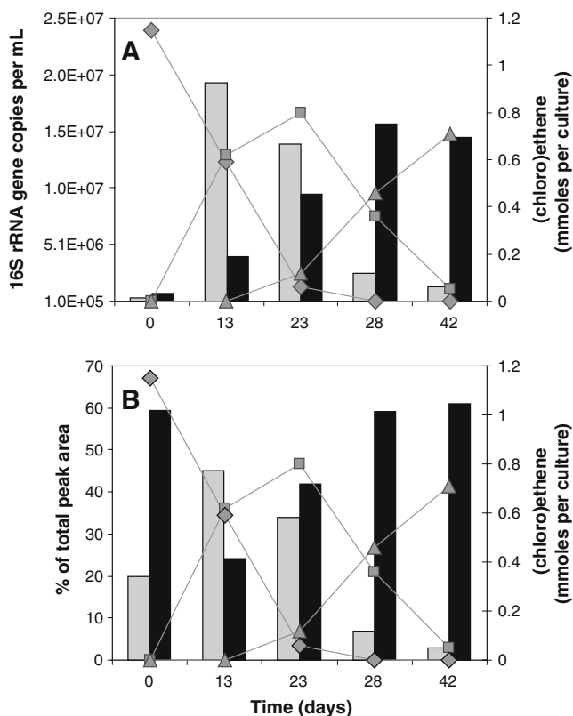
Fig. 2 Number of 16 S rRNA gene copies per mL of culture as determined by qPCR (a) and relative population sizes as determined by T-RFLP (b) of Desulfitobacterium spp. and Dehalococcoides spp. in an AQ1 enrichment culture dechlorinating cis -DCE to ethene with propionate-butyrate-ethanol as electron donors. For Dehalococcoides spp. the relative peak area of T-RF 168 is depicted, for Desulfitobacterium spp. the peak area represents the sum of the peaks of T-RF 212 and T-RF 329. Gray bars, Desulfitobacterium spp.; black bars, Dehalococcoides spp.; filled diamond, cis -DCE; filled square, VC; filled triangle, ethene
