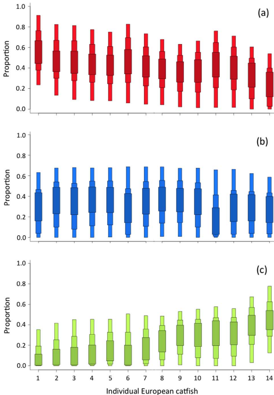
Figure 3. Predicted contribution of putative prey to the diet of each European catfish. Putative prey are (a) fish (in red), (b) crayfish (in blue) and (c) pigeons (in green). Reported values are the lower and upper 50, 75 and 95% Bayesian credibility intervals predicted by the mixing models.
