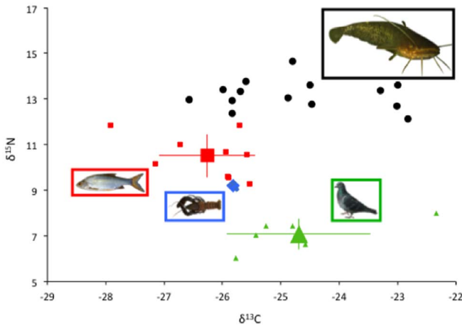
Figure 2. Stable isotope values of European catfish and the putative prey. \delta^{13}\text{C} and \delta^{15}\text{N} values (‰) of each individual ( n = 14 ) and the putative aquatic (fish, n = 9 and crayfish, n = 3 ) and terrestrial (pigeon, n = 6 ) prey are displayed. The large symbols for each prey represent the mean value ( \pm SD).
