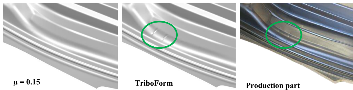
Figure 6. Simulated and actual part shape after forming showing wrinkles on the addendum
