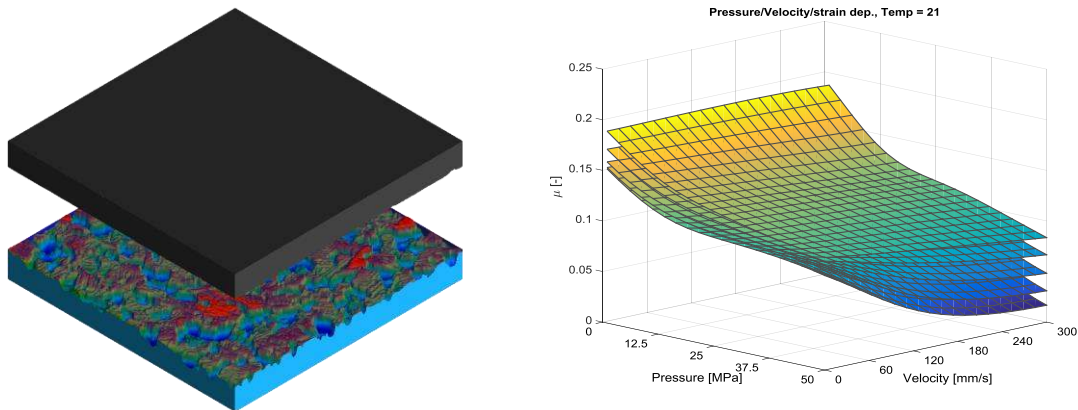
Figure 3. Projection of the die surface- and lubricated sheet surface topography in the TriboForm software (left) and the simulated friction behavior (right)
