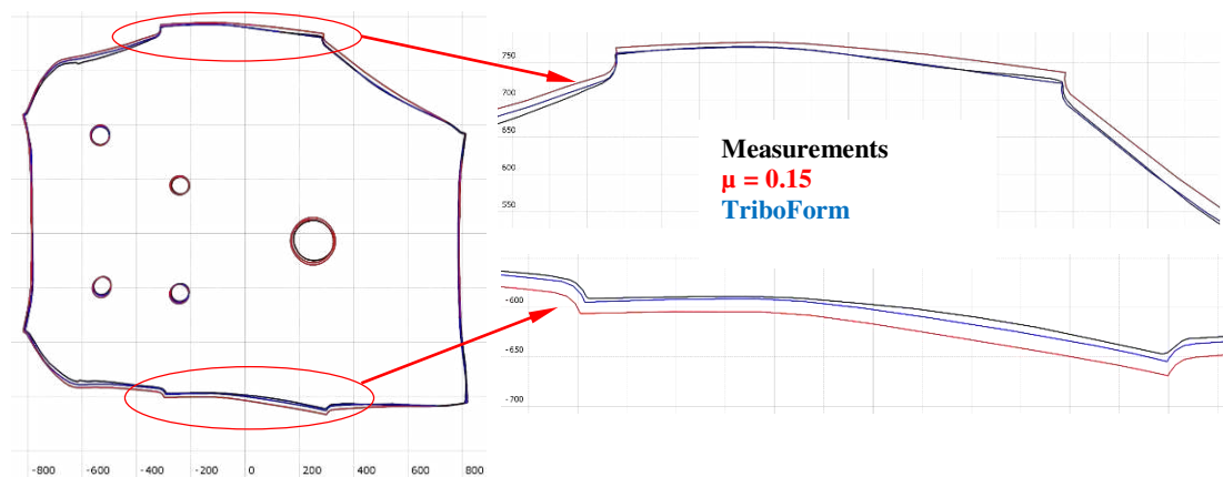
Figure 5. Experimentally measured and simulated draw-in results for the door inner part
