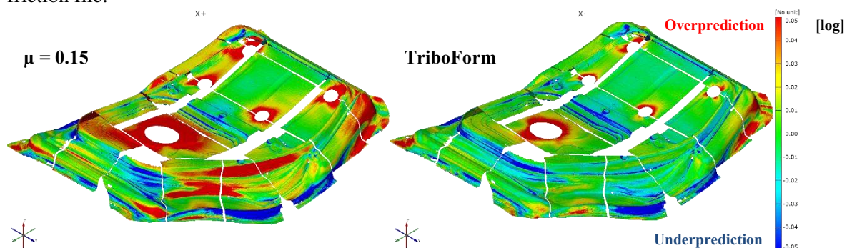
Figure 4. Difference in true major strain between simulations and experimental measurements.
