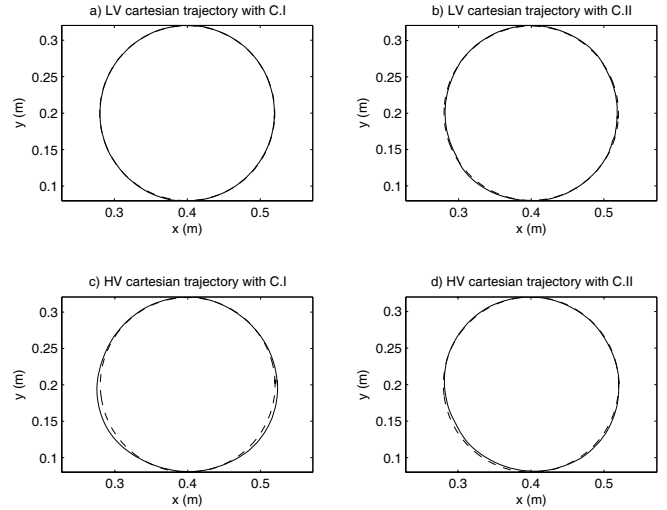
Fig. 1. Comparison of the experimental results: reference (dashed line) and tracked (solid line) trajectory with C.I and C.II in the LV and HV tests.
