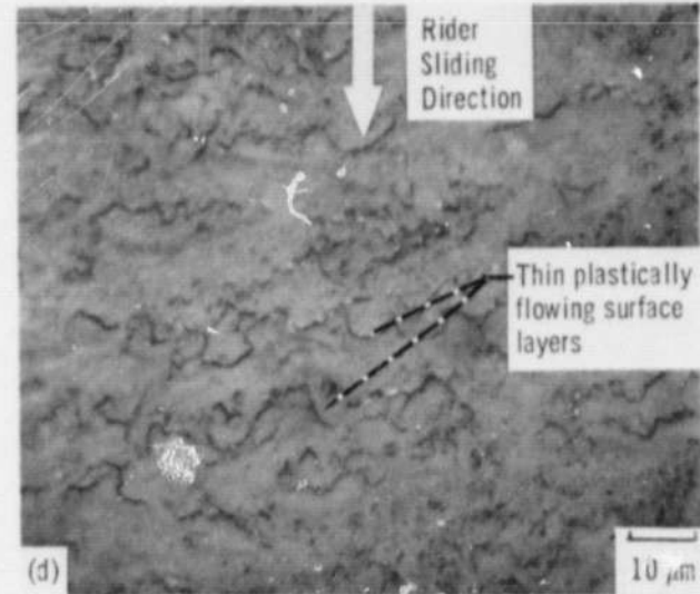
(b) Wear grooves and back transfer. (d) Plastically flowing surface layers.
