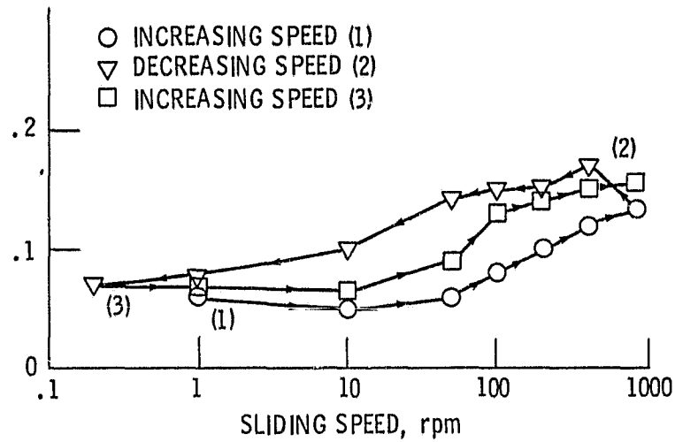
Figure 3. - Average friction coefficient as a function of sliding speed for a hemispherically tipped 440C HT stainless steel pin sliding against a UHMWPE disk at ambient temperature (25 o C) under a 9.8 N load in a 50% relative humidity air atmosphere. Sliding time at each speed was 5 minutes.
