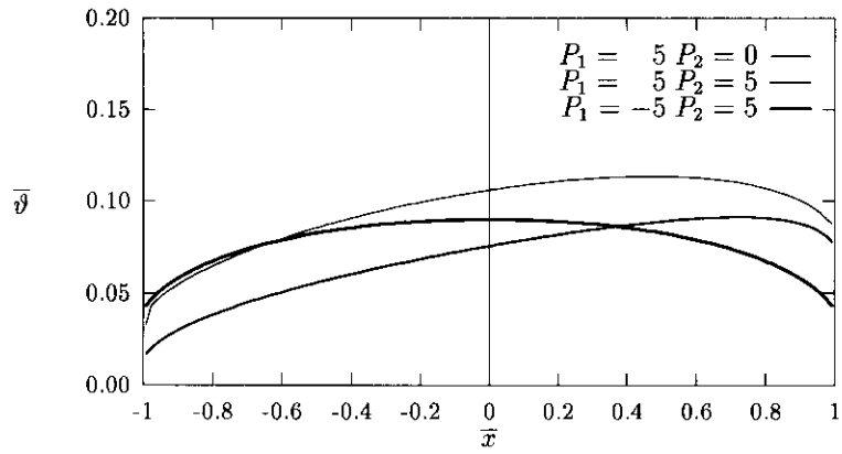
Figure 3.5: Center-line temperatures for different Péclet numbers, uniform heat source, \lambda = 1 .
