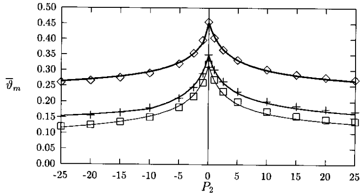
Figure 4.3: Dimensionless bulk temperature difference for F = F_m and a circular contact. Markers denote numerically calculated values. The lines represent the curvefit function. \diamond : P_1 = 1 ; + : P_1 = 10 ; \square : P_1 = 25 , \lambda = 1
