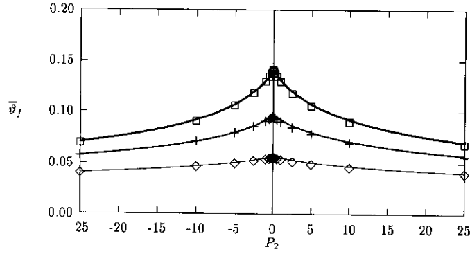
Figure 3.8: Maximum temperature, uniform heat source. Markers denote numerically calculated values. The lines represent the curvefit function. \diamond : P_1 = 50 ; + : P_1 = 10 ; \square : P_1 = 1 , \lambda = 1
