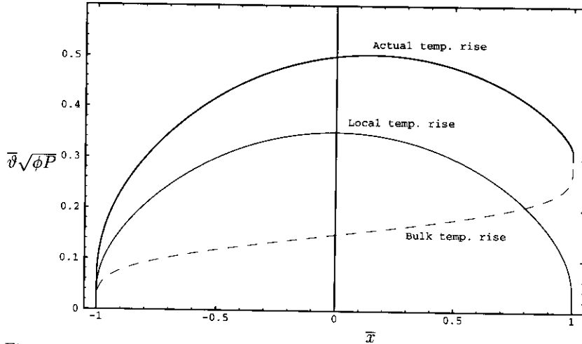
Figure 5.2: Centerline solution for local, bulk and actual contact temperature rise, semi-ellipsoidal heat supply ( \lambda = 1 ).
