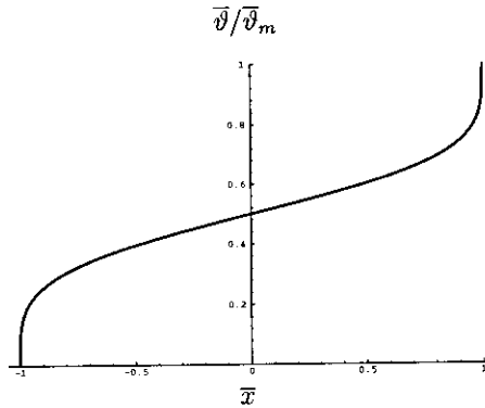
Figure 4.2: Temperature distribution at the line of symmetry for two equal bodies with equal high Péclet numbers, moving in opposite directions
