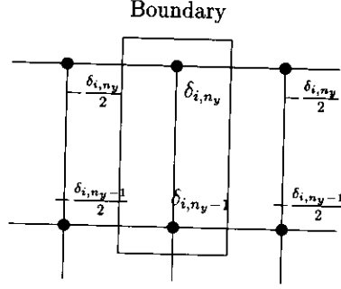
Figure 7.6: Distribution of the simultaneously calculated changes \delta_{i,n_y} and \delta_{i,n_y-1}
