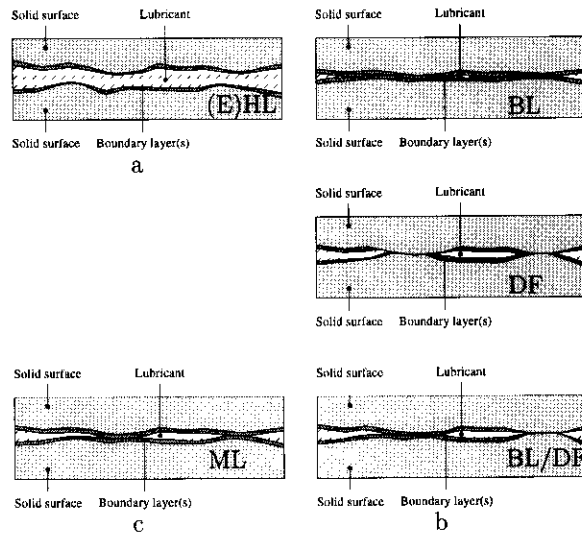
Figure 1.3: Lubrication modes
