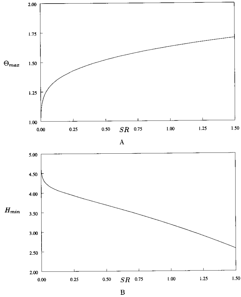
Figure 7.10: Film thickness and temperature rise as function of the slide to roll ratio for the conditions given in table 7.2. A: Maximum dimensionless contact temperature, B: Moes' dimensionless minimum film thickness parameter.
