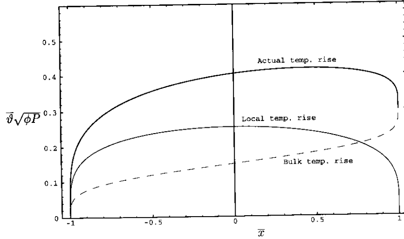
Figure 5.1: Centerline solution for local, bulk and actual contact temperature rise, uniform heat supply ( \lambda = 1 ).
