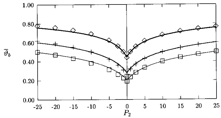
Figure 4.4: Average dimensionless contact temperature rise, due to a dimensionless bulk temperature difference of 1. Markers denote numerically calculated values. The lines represent the curvefit function. \diamond : P_1 = 1 ; + : P_1 = 10 ; \square : P_1 = 25 , \lambda = 1
