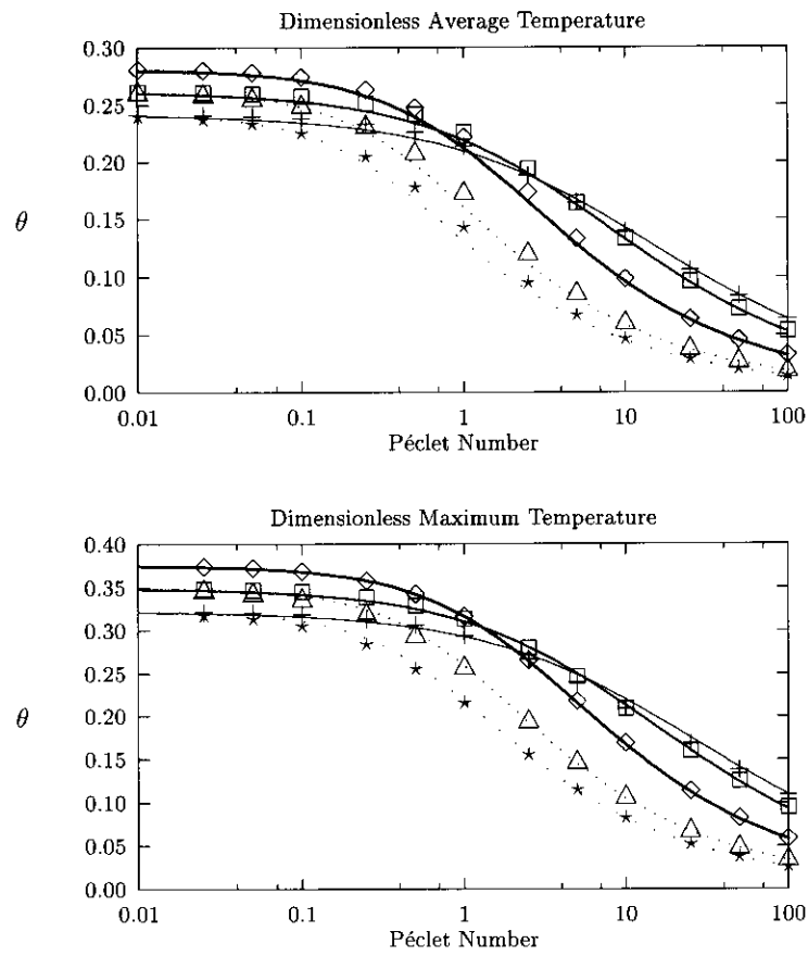
Figure 2.7: Average- and maximum temperature, semi-ellipsoidal heat source. Markers denote numerically calculated values. The lines represent the curvefit function. + : \phi = 1/5 , □ : \phi = 1/3 , ◇ : \phi = 1 , △ : \phi = 3 , * : \phi = 5 .
