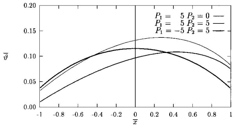
Figure 3.6: Center-line temperatures for different Péclet numbers, semi-ellipsoidal heat source, \lambda = 1 .
