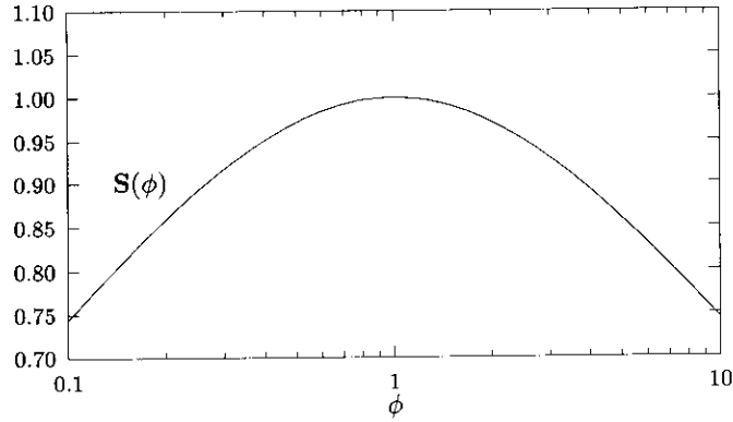
Figure 2.5: The shape factor S(\phi) .
