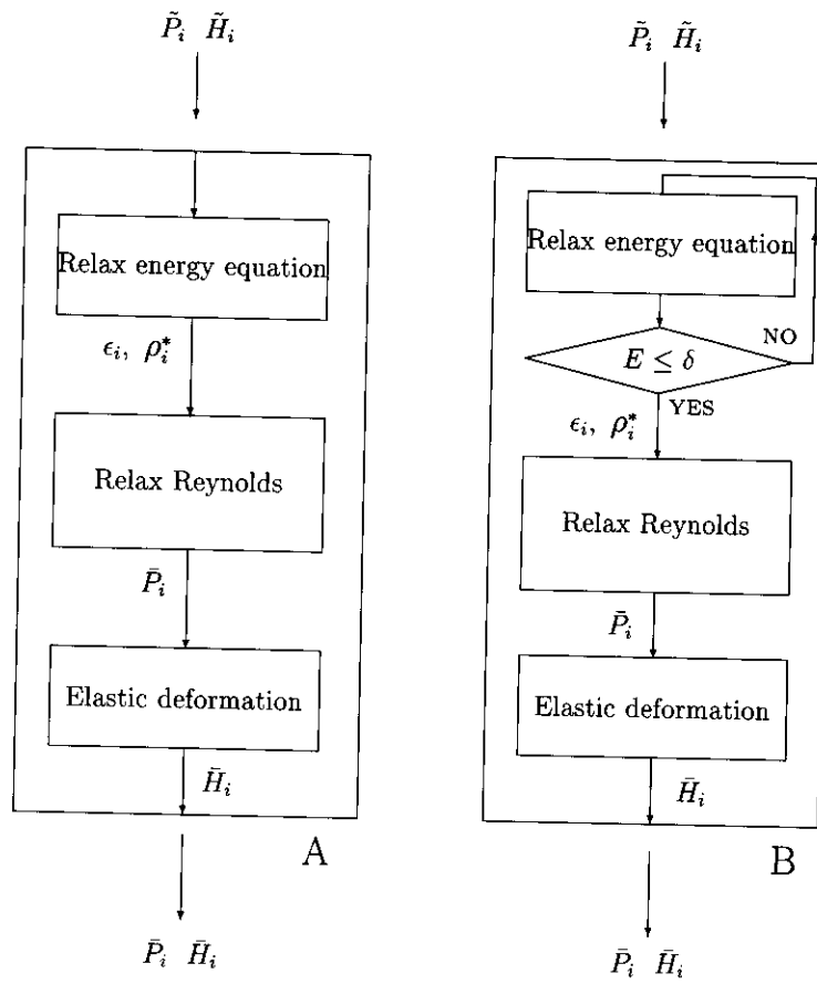
Figure 7.3: Flow diagram of the relaxation process as proposed (A), and the (computationally inefficient) alternative with a nested loop (B)
