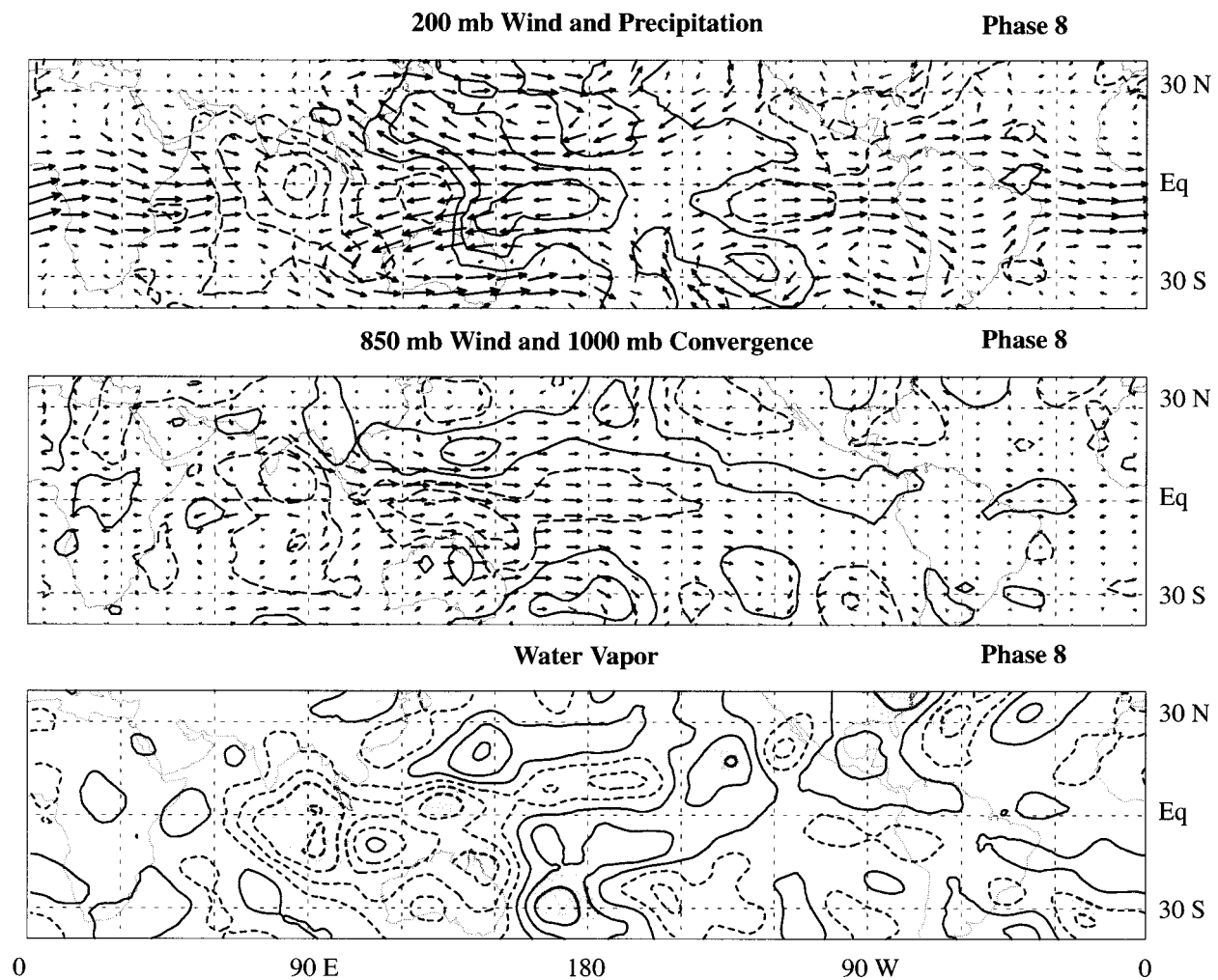
FIG. 13. Same as Fig. 3 but for phase 8.
