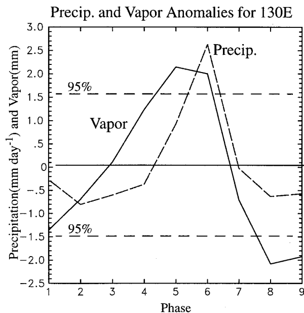
FIG. 11. Precipitation anomalies and water vapor anomalies for the years 1988–92 (all seasons) as a function of phase for a 5^{\circ} \times 5^{\circ} box centered at the equator and 130^{\circ}\text{E} : precipitation (dashed) and vapor (solid). The dotted horizontal lines are the limits at which the water vapor signal is significantly different from zero at the 95% level.
