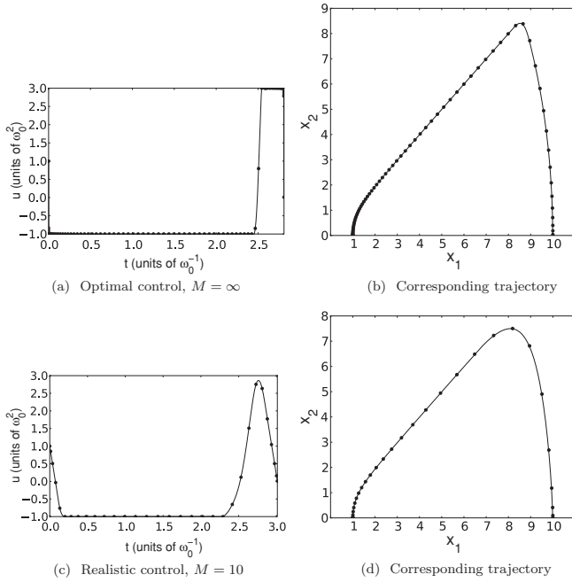
FIG. 7. Control functions calculated by the pseudospectral method for the same parameters as in Fig. 2 without [ M = \infty , (a)] and with [ M = 10 , (c)] slope restriction. The latter case requires a larger transfer time, as expected. The corresponding trajectories are also shown (b, d).
