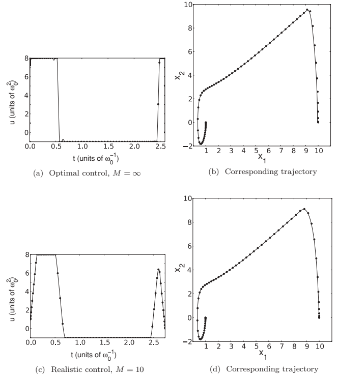
FIG. 8. Control functions calculated by the pseudospectral method for the same parameters as in Fig. 3 without [ M = \infty , (a)] and with [ M = 10 , (c)] slope restriction. The latter case requires a larger transfer time, as expected. The corresponding trajectories are also shown (b, d).
