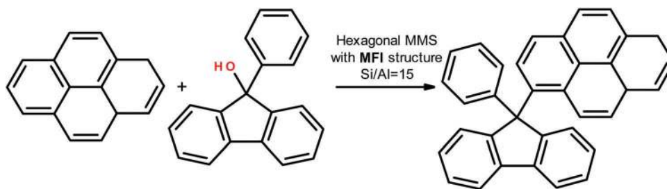
Scheme 2 Alkylation of pyrene with 9-phenyl-9-fluorenol.
