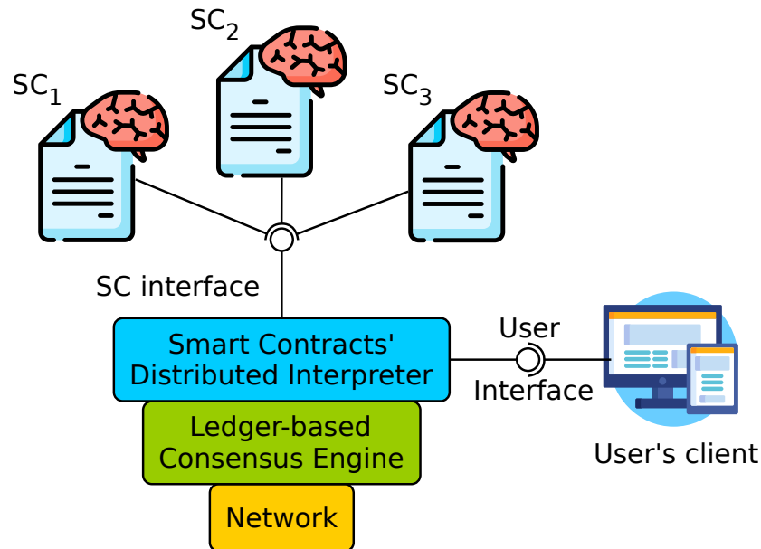
Figure 4. General layered architecture of smart contract (SC)-enabled blockchain technology (BCT).
