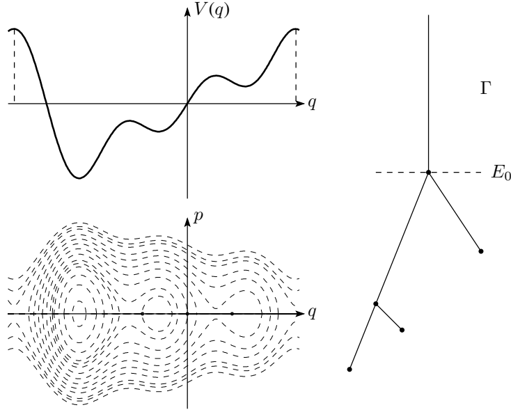
Figure 2: Example of a potential with the orbits of the Hamiltonian flow and the corresponding Freidlin-Wentzell graph \Gamma .
