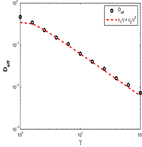
Figure 3: Large \gamma asymptotic for the effective diffusivity.
