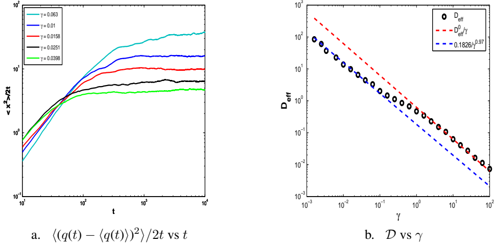
Figure 1: Second moment and effective diffusivity for various values of \gamma .
