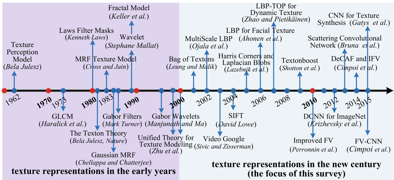
Fig. 2 The evolution of texture representation over the past decades (see discussion in Sect. 2.2)
