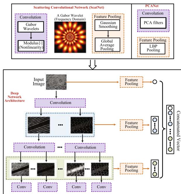
Fig. 21 Illustration of two similar handcrafted deep convolutional networks: ScatNet (Bruna and Mallat 2013) and PCANet (Chan et al. 2015)
