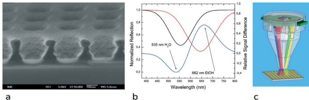
Fig. 5 (a) A scanning electron microscopy image of the substrate for measuring surface plasmon resonance. (b) Left axis: normalized amplitude of reflected light from the LSPR chip covered with H 2 O (black) or ethanol (red). Right axis: the blue line shows the difference between both curves. (c) CAD design of the LSPR head.
