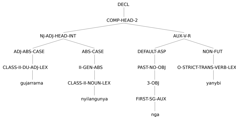
FIGURE 6.: Treebank tree format for (1)
