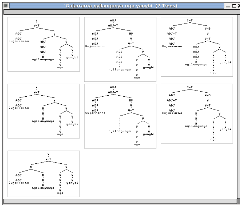
FIGURE 4.: Seven analyses of (1)
