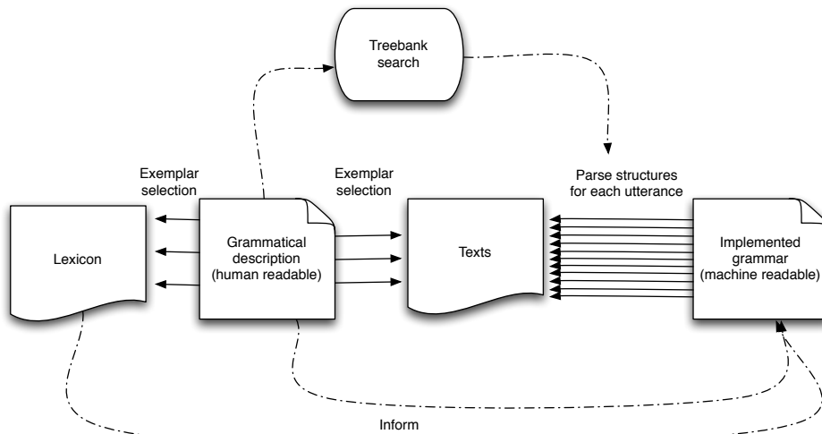
FIGURE 2.: Schematic view of electronic grammars with treebanks
