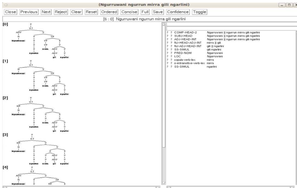
FIGURE 5.: Treebanking tool
