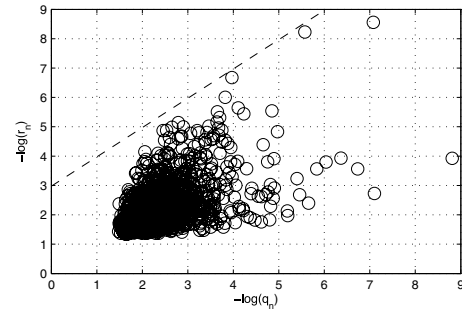
Fig. 1. The Ignorance -\log [r_n(Y_n)] (ECMWF ensemble and climatology) versus -\log [q(Y_n)] (only climatology) for temperature at Heligoland, German Bight (WMO 10015), lead time ten days. The dressing method here is AKD. Obviously, -\log [r_n(Y_n)] is never larger than -\log [q(Y_n)] - \log(1 - \alpha) . The weight assigned to the climatology is 1 - \alpha = 0.051 , whence -\log(1 - \alpha) \approx 3 .
