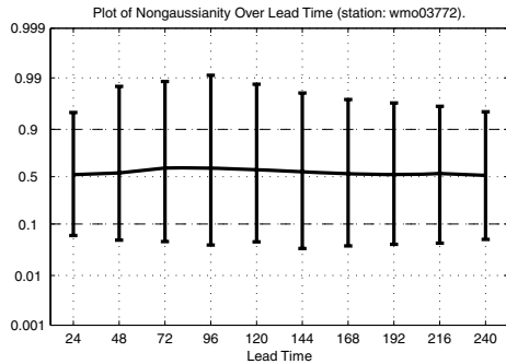
Fig. 6. The 10–90% range of the \kappa -statistic for London Heathrow. The y-axis is calibrated in terms of quantiles of the \kappa -statistic for Gaussian ensembles and plot on \log(\frac{p}{1-p}) scale.
