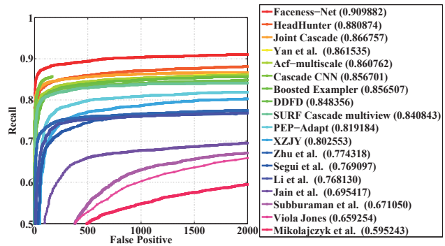
Figure 10. FDDDB results. Recall rate is shown in the parenthesis.
