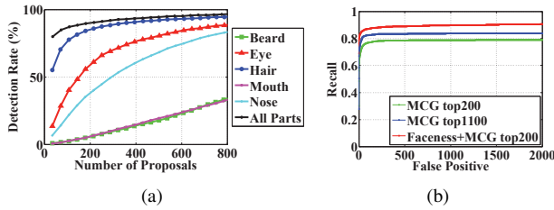
Figure 8. (a) Contribution of different face parts on face proposal. (b) FDDDB face detection results with different proposal methods.
