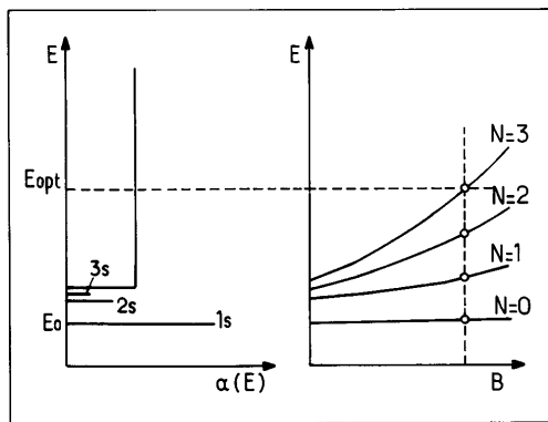
FIG. 1. Scheme of the electron-hole pair excitations in a semiconductor quantum well at zero magnetic field (left), and in presence of a quantizing magnetic field B applied along the growth axis (right). E_0 is the energy of the 1s Wannier exciton ground state.
