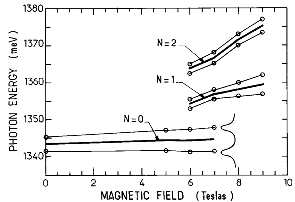
FIG. 4. Energies of the reflectivity doublets at resonance observed in Fig. 3, plotted against the magnetic field B (open circles). The solid lines are guides to the eye showing the fan chart of magneto-optical transitions.
