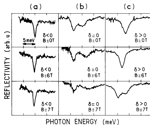
FIG. 2. Selected reflectivity spectra for various detuning energies \delta and various magnetic fields B .
