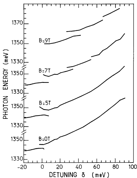
FIG. 3. Energies of the reflectivity peaks versus the detuning energy \delta , for various values of the magnetic field B .
