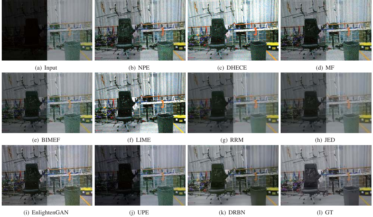
Figure 3. The visual results of different methods. Left part: the original results. Right part: the results corrected by Gamma transformation for better visibility.
