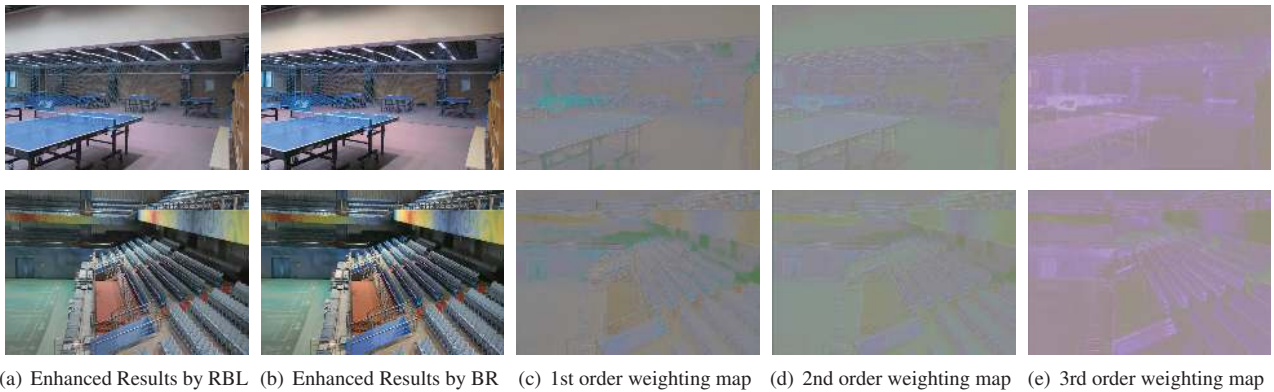
Figure 7. The visualization results of the learned weighting maps for band recombination. RBL and BR denote the recursive band learning and band recombination, respectively.
