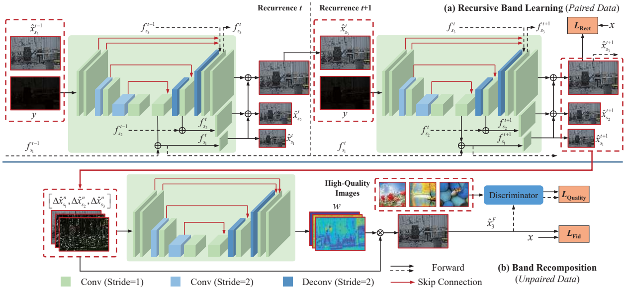
Figure 2. The framework of the proposed Deep Recursive Band Network (DRBN), which consists of two stages: recursive band learning and band recomposition. (1) In the first stage, a coarse-to-fine band representation is learned and different band signals are inferred jointly in a recursive process. The enhanced result from the last recurrence is used as the guidance of the next recurrence and the later recurrence is only responsible to learn the residue in the feature and image domains at different scales. (2) In the second stage, the band representation is recomposed to improve perceptual quality of the enhanced low-light image via a perceptual quality-guided adversarial learning.
