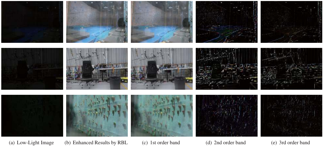
Figure 6. The visualization results of the learned bands by our DRBN. RBL denotes the recursive band learning.
