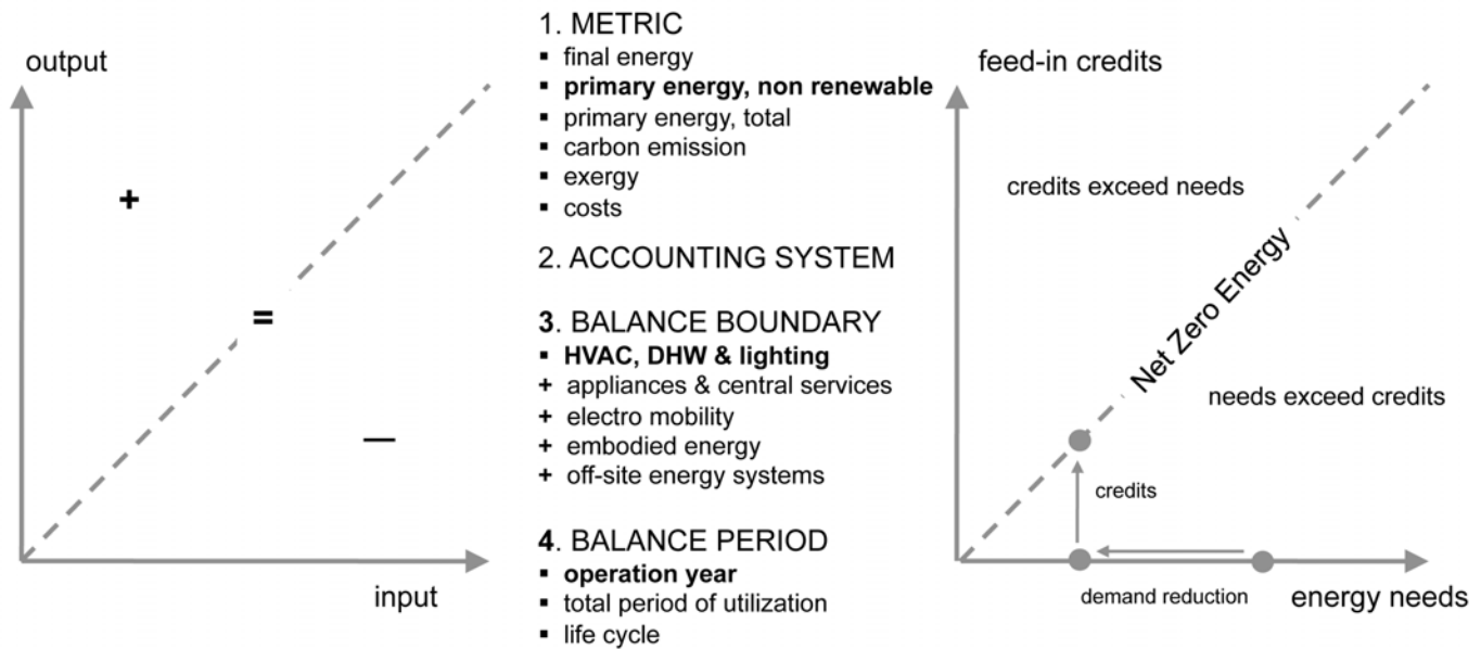
FIGURE 1. The left-hand diagram illustrates the schematic input/output balance of a building project. The balance calculation needs the definition of a metric and an accounting system, the system boundary and the balancing period. As an example, the right-hand diagram uses primary energy (non-renewable fraction only), the system boundary of the German energy code EnEV and one year of operation. The diagonal within the diagram describes a net zero-energy building in this context. The primary energy demands are balanced by the primary energy equivalent of the electricity fed into the local grid. Net plus-energy buildings in that sense are represented in the upper left part of the diagram.
