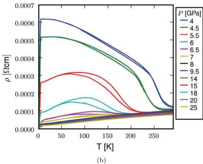
Figure 2: Resistivity in the pressure range of 0–25 GPa and temperature range of 1.3–300 K.
