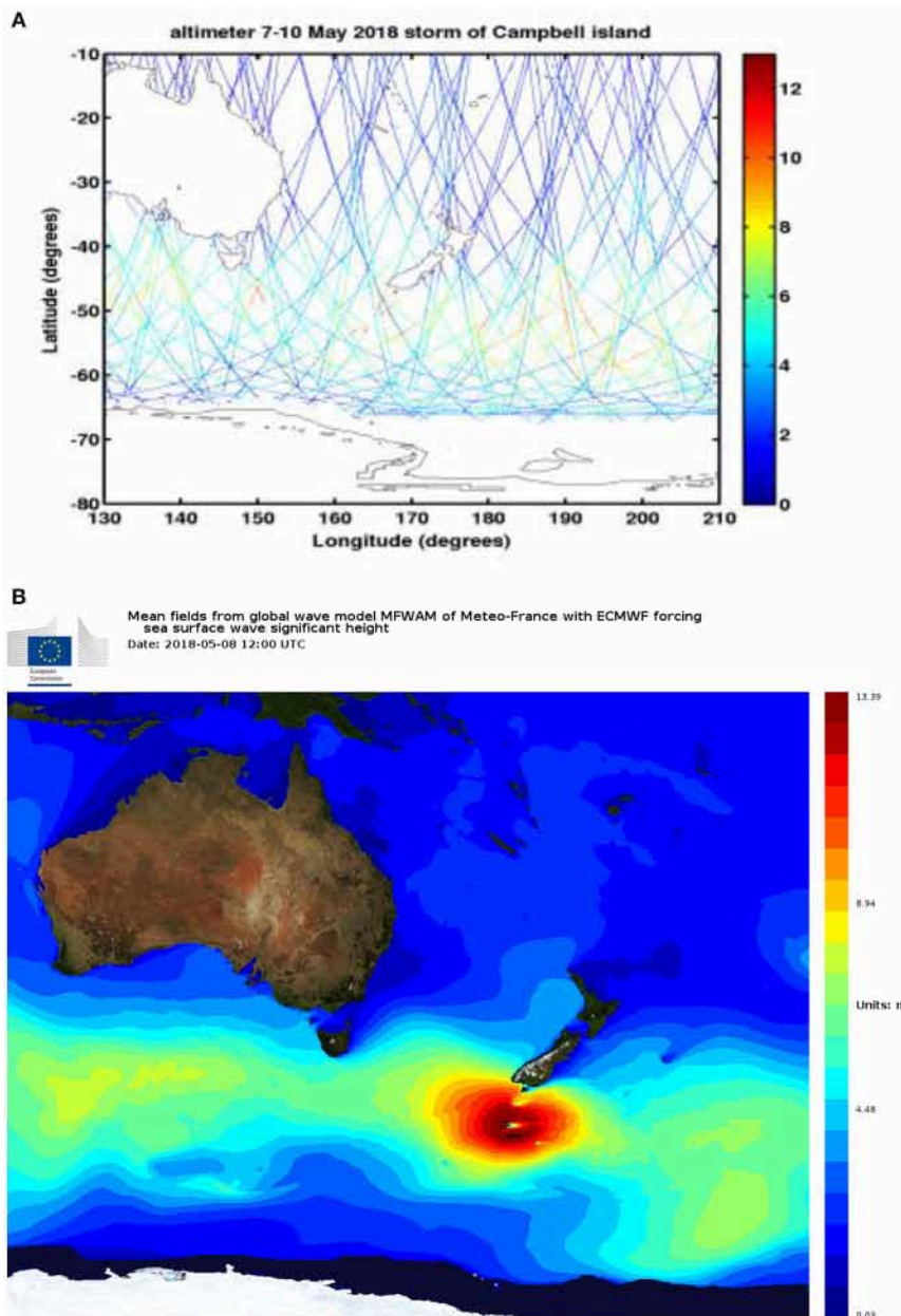
FIGURE 7 | (A) Significant wave heights on ground tracks from 5 altimeters during the storm at Campbell Island (south of New Zealand) from 7 to 10 May 2018. (B) Significant wave heights from the global CMEMS-MFC wave system on 8 May 2018 at 12:00 UTC. High waves induced by a severe storm, with SWH of 13.8 meters at Campbell Island south of New Zealand.
