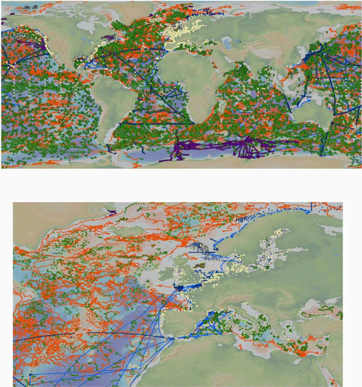
FIGURE 8 | Data at INS-TAC for Spring (January-March) 2018. Argo (green), vessels (XBT and CTD, thermosalinographs (blue), sea mammals (purple), gliders (yellow), moorings, tide gauges and rivers (white) (global and zoom on European seas).
