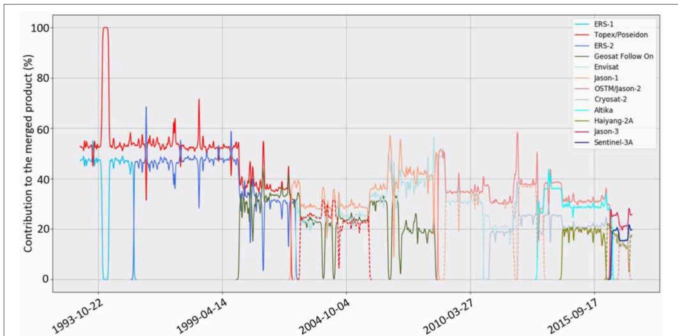
FIGURE 3 | Relative contribution (in percent) of each altimeter mission in the CMEMS multi-mission altimeter maps. Results are derived from a Degrees of Freedom of the System analysis. The top-right legend details the name of the altimeter missions in chronological order. In several cases, when the orbit configuration changes (e.g., management at the end of life of the mission) the mission contribution is represented by a dashed line.
