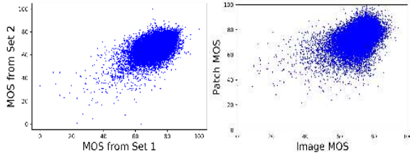
Fig. 7: Scatter plots descriptive of the new subjective quality database. Left: Inter-subject scatter plot of a random 50% divisions of the human labels of all 40K+ pictures into disjoint subject sets. Right: Scatter plot of picture MOS vs MOS of largest patch (40% of linear dimension) cropped from each same picture.
