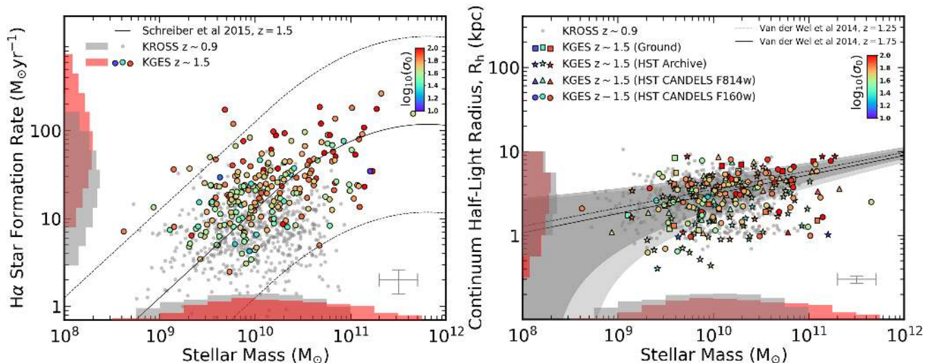
Figure 2. Left panel: The extinction corrected H \alpha star formation rate for the KGES sample as a function of stellar mass as derived from SED fitting using MAGPHYS (da Cunha et al. 2008). The KROSS z \sim 0.9 sample is shown as grey points in the background. The Schreiber et al. (2015) z = 1.5 star-formation rate stellar mass tracks, converted to a Chabrier IMF, are shown as well as factor 10 above and below the model track. Right: Stellar continuum half-light radii, derived from GALFIT, as a function of stellar mass. KROSS z \sim 0.9 sample shown as grey points in the background. Ground ( H , K ) imaging (squares), non-CANDELS HST imaging (stars), CANDELS HST F814W imaging (triangles) and, CANDELS HST F160W imaging (circles). The dashed and solid lines indicate the mass-size relation for star-forming galaxies at z = 1.25 and z = 1.75 respectively, as derived by van der Wel et al. (2014), with the shaded region indicating the uncertainty on the relations. The median uncertainty on stellar mass, star formation rate and stellar continuum size are shown by grey bars in the lower right corner of each panel and the distribution of velocity dispersion within the sample is shown by the colour bar. In both panels we show histograms of each observable for both KROSS and KGES surveys. The figure indicates that the star-formation rates and stellar continuum sizes of the KGES galaxies are ‘typical’ of star-forming galaxies at z \sim 1.5 .
