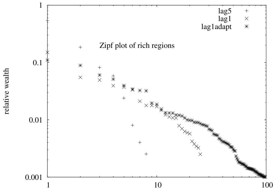
Figure 8: Zipf plot of wealth of the most active regions for the standard and adaptive firms models (cf. section 4.1). The vertical axis display the production relative to the total production. The '+' signs correspond to the standard model with time lag = 5, the 'x' to time lag = 1, and the '*' to the adaptive firms model with time lag = 1.
