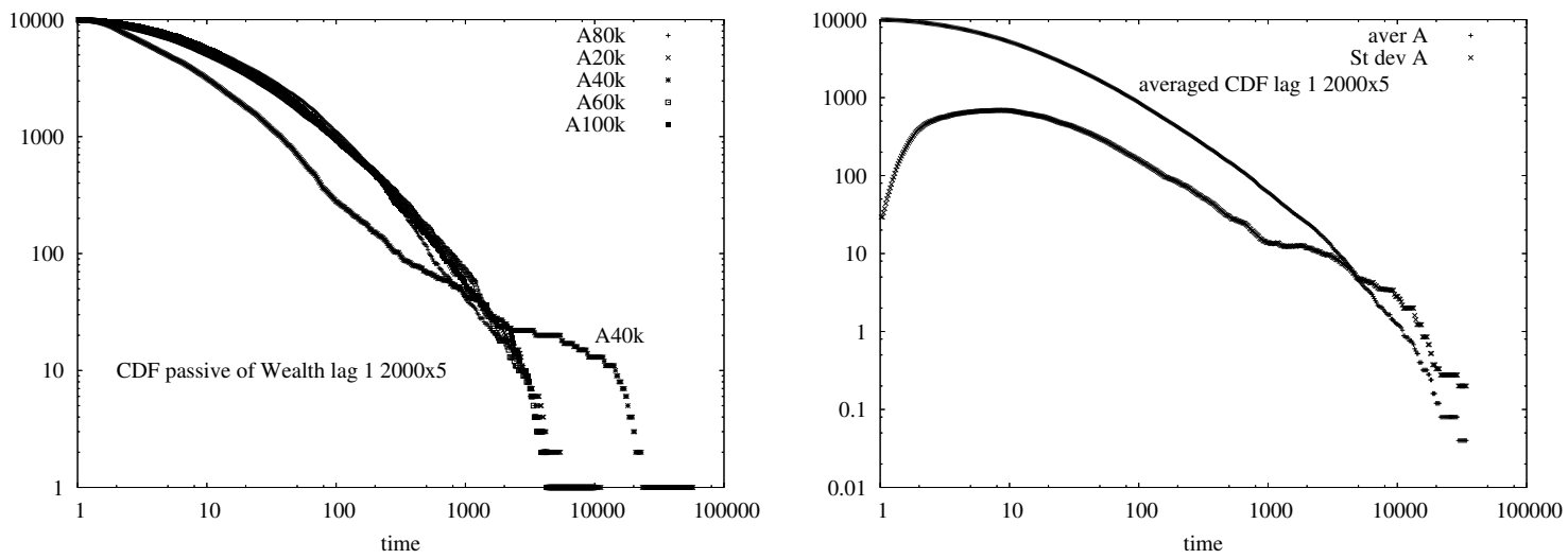
Figure 9: Cumulative distributions of wealth in the absence of avalanches, after several ten thousands iteration steps. Left diagrams are series of histograms at different times: even after long evolution, the distribution may still fluctuate by large amounts. Right diagrams: time averaged and standard deviation of histograms. Parameter choices are the same as for the previous figures.
