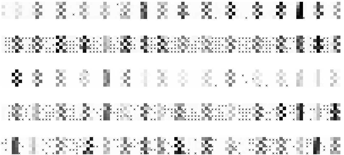
Figure 11: Series of wealth and patterns for a network of "adaptive" firms. The conventions and parameters are the same as for figures 5 and 6, for a 100x5 lattice. Time lag is 1. Patterns are taken at time 2000 (for the lower pattern) and 4000, 6000, 8000, 1000 upward. The position of the rich regions are stable, but their relative amplitude varies.
