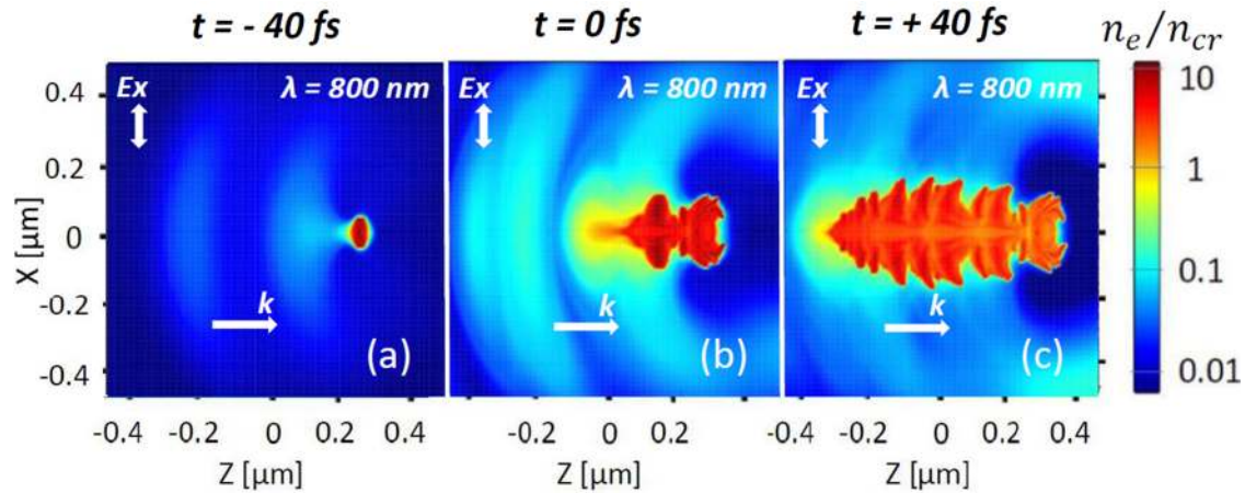
FIG. 1. Electron density snapshots are calculated by coupled 2D-FDTD (1)–(5) demonstrating the evolution from a single inhomogeneity of radius a = 5 nm localized in (0.3, 0) \mu\text{m} to nanoplasmic taken at (a) 40 fs before the pulse peak, (b) at the pulse peak, and (c) 40 fs after the pulse peak. Laser irradiation conditions: pulse duration \theta = 120 fs (FWHM), irradiation wavelength \lambda = 800 nm, pulse energy E = 300 nJ. Here and further, electron density is normalized to its critical value at 800 nm n_{\text{crit}} = 1.7 \times 10^{27} \text{m}^{-3} and \vec{k} is the incident laser wave vector.
