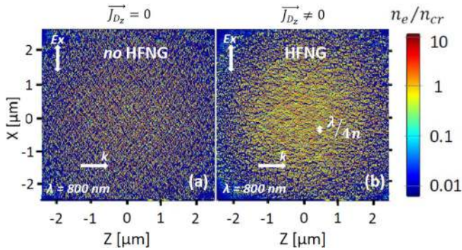
FIG. 6. Electron density snapshots are obtained by coupled 2D-FDTD (1)–(5) assuming (a) J_{D_z} = 0 and (b) J_{D_z} \neq 0 at the end of the pulse duration \theta = 240 fs (FWHM), laser wavelength of 800 nm and pulse energy of 500 nJ with initial concentration of inhomogeneities C_i = 9\% . The schematic representation of the initial distribution of inhomogeneities is shown in Fig. 2(b).
