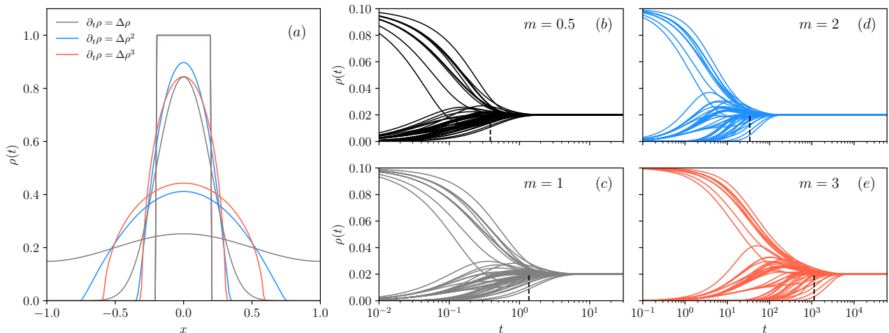
FIG. 1: Nonlinear diffusion yields mass propagation at a finite speed, in contrast with linear diffusion. (a) PME in a box of length two with no-flux boundary conditions and for exponents m = 1, 2, 3 – m = 1 corresponds to the linear diffusion equation. Solutions at three different time points starting from a compactly supported initial condition. Note the slower decay of the PME for exponents m = 2, 3 . (b)-(e) Numerical solutions of Eq. (13) with \lambda = 1 , for an Erdos-Renyi network with M = 50 and a probability of drawing any possible edge p = 0.1 . The four numerical simulations start from the same initial conditions and take place on the same network. At t = 0 , 10 randomly selected nodes start with \rho_i = 0.1 , so \bar{\rho} = 1/M . Dashed lines correspond to the relaxation time given by Eq. (26).
