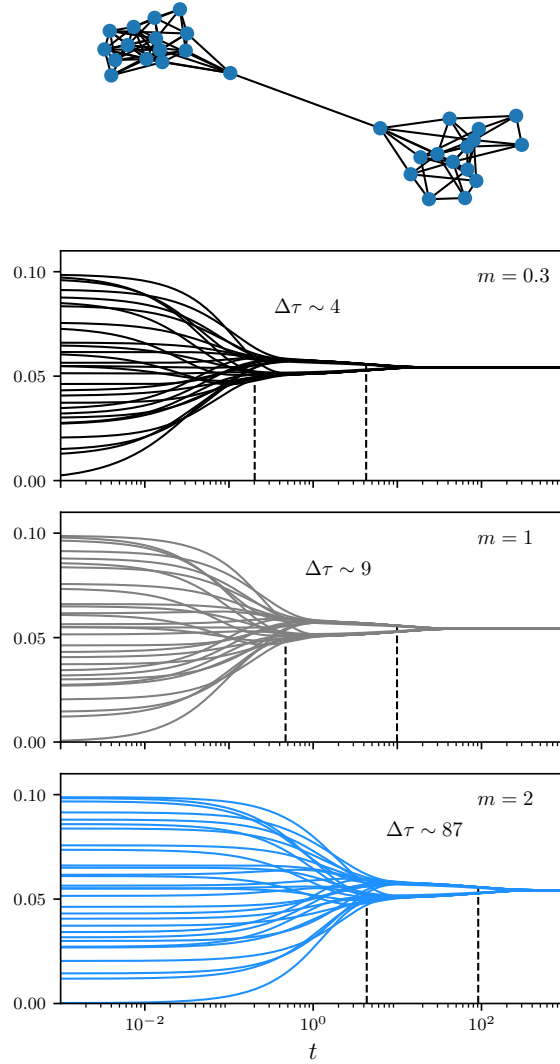
FIG. 3: Nonlinear diffusion on modular networks. Here we use a network with two large components with M = 15 nodes each, and an edge that serves as a link. For every numerical simulation \bar{\rho} = 0.05 , \lambda = 1 . Dashed lines represent the times \tau_1 and \tau_2 .
