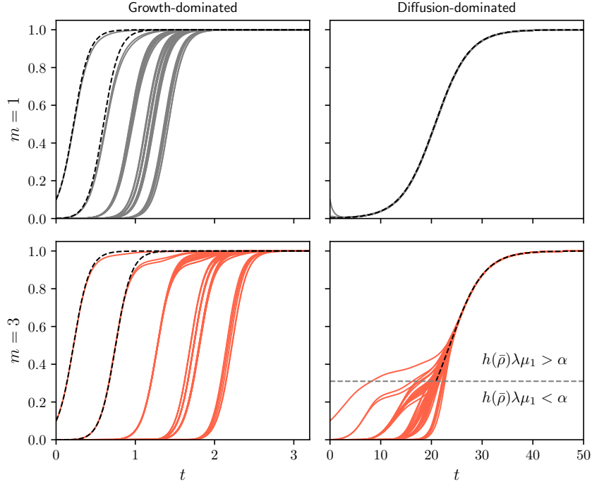
FIG. 4: A Fisher-KPP type equation in the growth-dominated regime (left, \lambda = 0.05 , \alpha = 10 ) and the diffusion-dominated regime (right, \lambda = 1 , \alpha = .3 ): comparing linear (top) with nonlinear diffusion with exponent m = 3 (bottom). Simulations take place on Erdos-Renyi networks with a number of nodes M = 50 and a probability of drawing any possible edge p = 0.1 . Black dashed lines correspond to the asymptotic solutions derived in Appendix C. Gray dashed line is given by (29).
