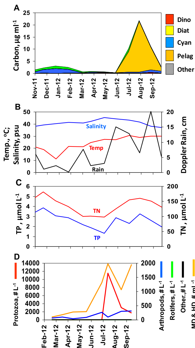
Fig. 15 Phytoplankton biomass divided into five major groups (top), i.e., dinoflagellates ( Dino ), diatoms ( Diat ), cyanobacteria ( Cyan ), Pelagophytes ( Pelag ), and other taxa (a); surface water temperature, salinity, and local doppler rainfall (b); total nitrogen and total phosphorus concentrations (c); potential grazers of phytoplankton were divided into five groups, i.e., protozoa, arthropods (e.g., copepods), rotifers, other zooplankton taxa, and potential mixotrophic, MD, and heterotrophic, HD, dinoflagellates; during the 2012 time period at the central ML site
