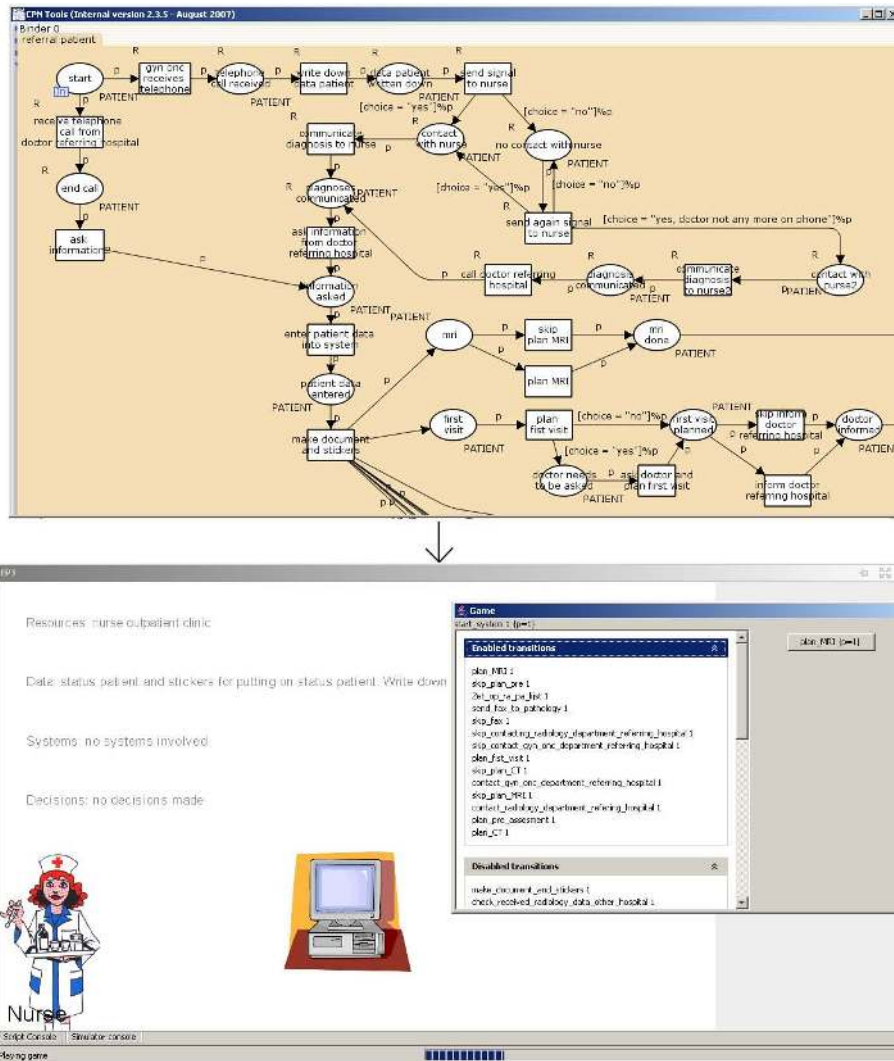
Fig. 3. Animation belonging to the “make document and stickers” activity. In addition, the panel at the top right side shows which activities are enabled now.
