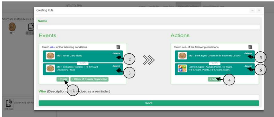
Fig. 7. Example of ECA rule created for the scenario “game in the archaeological park”.
