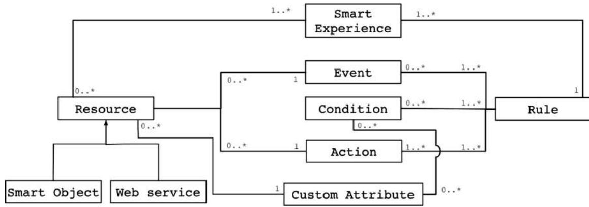
Fig. 1. A schematic representation of the main conceptual elements to compose smart experiences.
