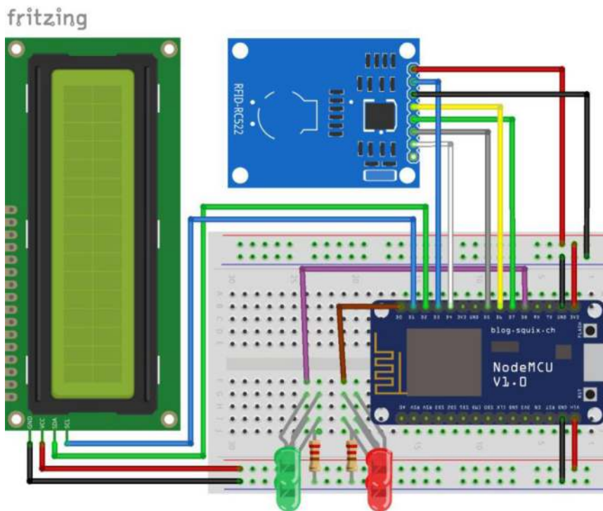
Fig. 5. Electric schema of the Mouth of the Truth used by the guide.
