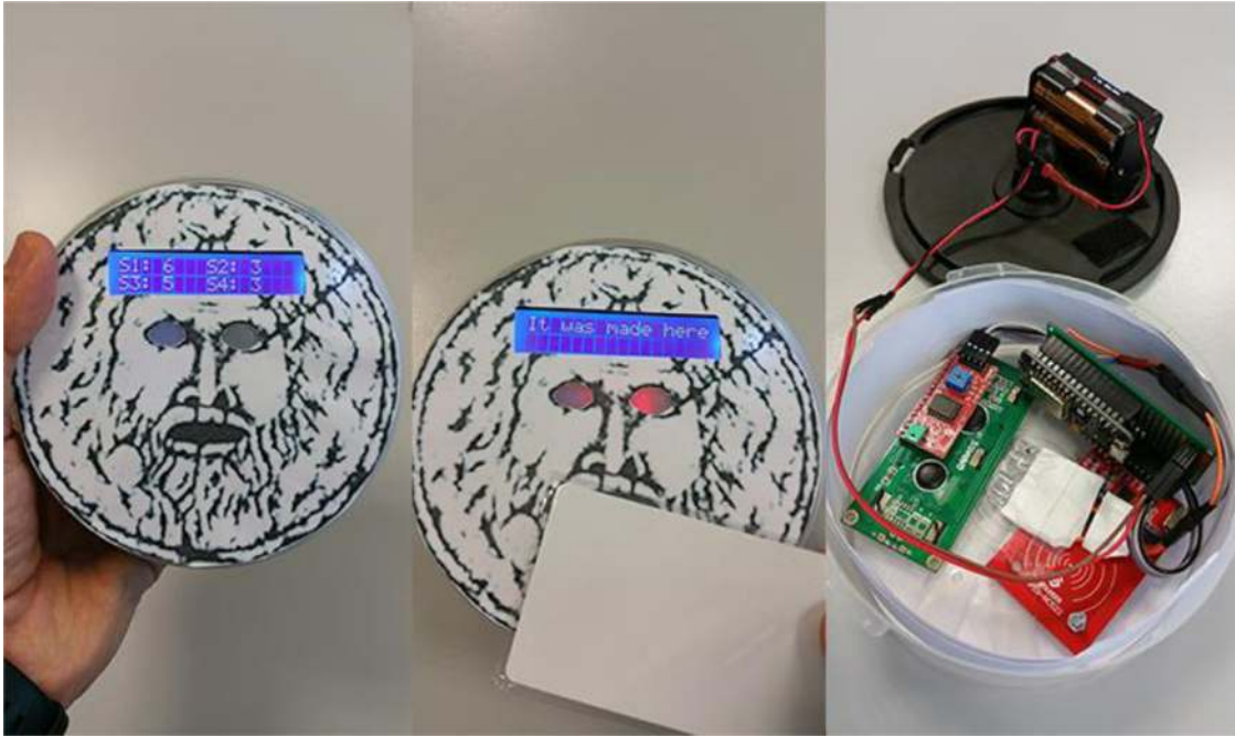
Fig. 4. The Mouth of Truth smart object built to develop the scenario “game in the archaeological park”.
