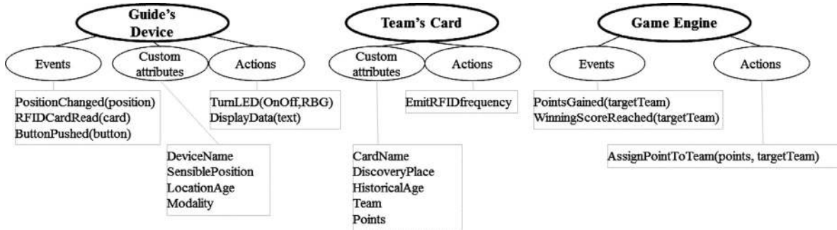
Fig. 2. Models of the smart objects and the Web service involved in the Rocco's scenario.
