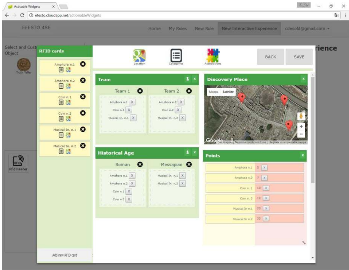
Fig. 6. Defining objects and their attributes for the scenario “game in the archaeological park”.
