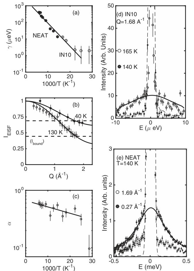
FIG. 2. The quasielastic linewidth (a), momentum dependence (b), and the elastic fraction (c) are plotted for \text{CH}_3\text{NH}_3\text{PbBr}_3 . Sample quasielastic scans and fits are shown from the IN10 backscattering spectrometer (d) and the NEAT direct-geometry time-of-flight spectrometer (e).
