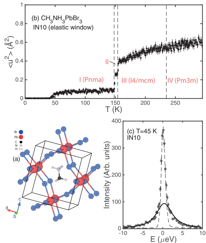
FIG. 1. (Color online) (a) The structure of \text{CH}_3\text{NH}_3\text{PbBr}_3 illustrating the MA molecular cations in the \text{PbBr}_3 framework at 5 K. (b) shows the mean-squared displacement of the hydrogen atoms ( \langle u^2 \rangle ) extracted from an IN10 elastic window scan as a function of temperature and (c) plots a representative quasielastic scan taken on IN10 at 45 K.
