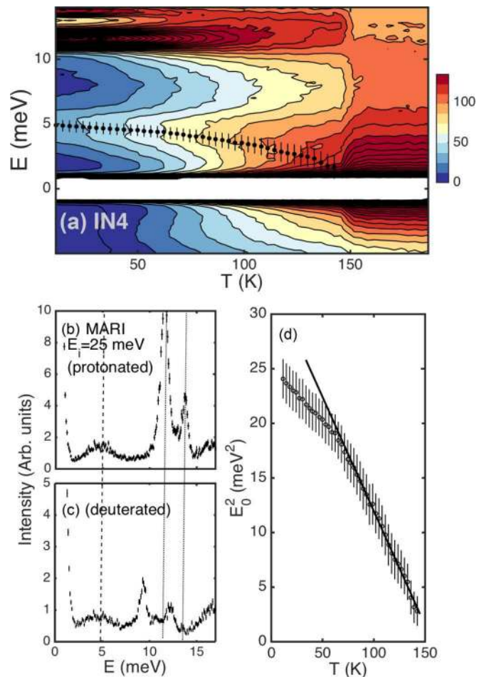
FIG. 3. (Color online) (a) displays inelastic scans taken on the IN4 spectrometer. (b) and (c) show momentum integrated scans on MARI on fully protonated and deuterated samples. (d) shows a plot of the square of the \text{PbBr}_6 octahedra phonon frequency as a function of T .
