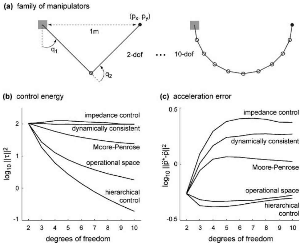
Figure 4. Comparison of control methodologies on a family of robotic manipulators.
