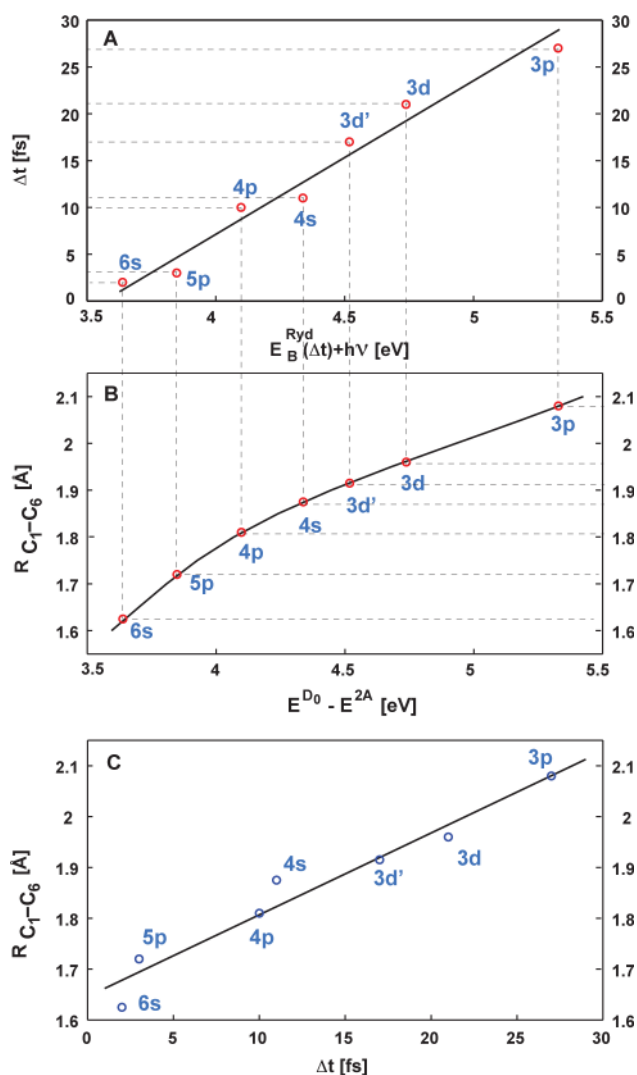
Figure 7. (A) Experimentally measured travel times of the wavepacket on the 2A surface to the resonance window for photoionization via the observed Rydberg states as a function of the combined binding and photon energy (eq 3). (B) Calculated distance between the terminal carbon atoms, R_{C_1-C_6} , as a function of the energy difference between the 2A state and the ground state ion. The dashed lines in panels A and B connect the distance between the terminal carbon atoms and the travel time since the energy scales are equal (eq 3). (C) Derived structural parameter R_{C_1-C_6} as a function of wavepacket travel time.
