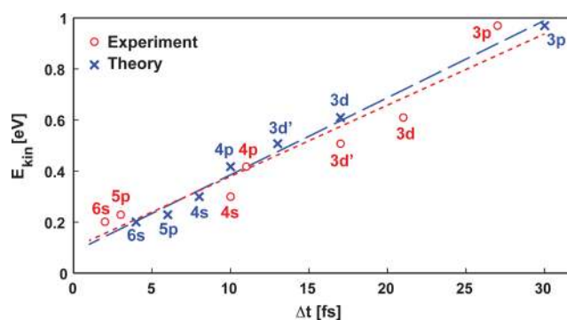
Figure 8. Kinetic energy of the wavepacket as a function of travel time in 2A as determined by the experiment (red circles and dotted line) and the computation (blue symbols and dashed line). Kinetic energies at the locations of the Rydberg state resonance windows, for both the experimental and calculated travel times, were obtained by subtracting the potential energy of 2A at the corresponding R_{C_1-C_6} (Figure 6), from the total energy deposited by the pump photon.
