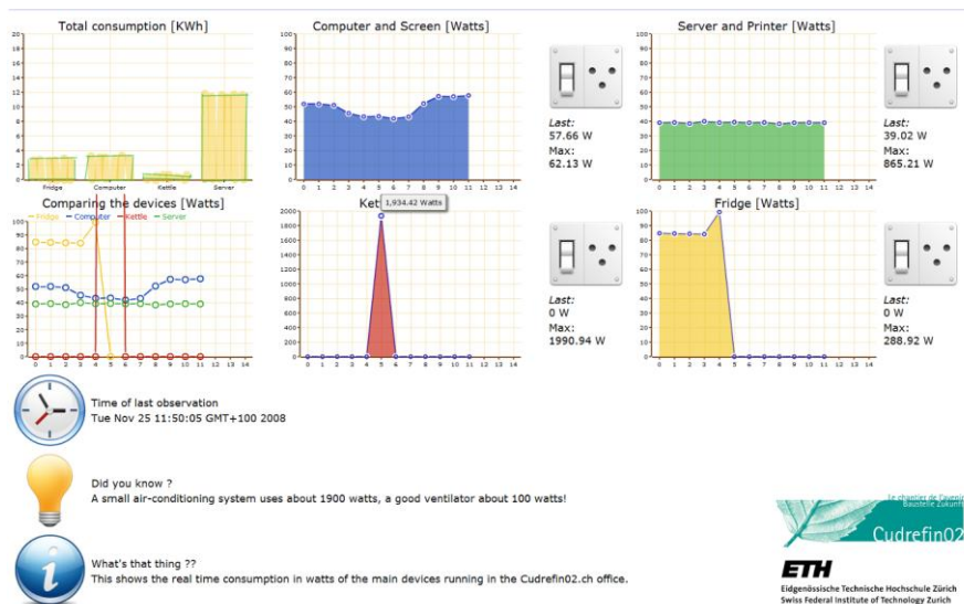
Fig. 5.5 The Web-Based User Interface for Monitoring and Controlling the Ploggs
