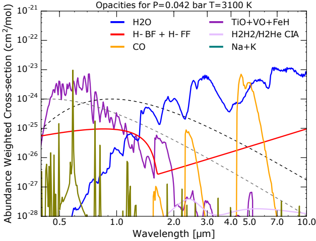
Fig. 4. Abundance weighted cross sections of relevant ions and molecules taken close to the 1.4\,\mu\text{m} photosphere of WASP-121b ( P = 40\text{ mbar} , T = 3100\text{ K} ). The dashed line represents a scaled blackbody emission curve at a temperature of 3100\text{ K} (black, corresponding to the planet emission) and 6460\text{ K} (gray, corresponding to the incoming stellar light).
